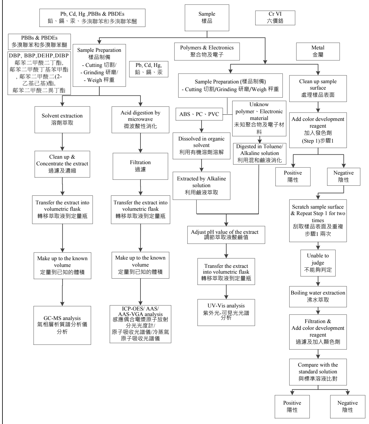
Test Flowchart of Heavy Metals, Flame Retardants and Phthalates Content [ European Council Directive 2011/65/EU ] :
