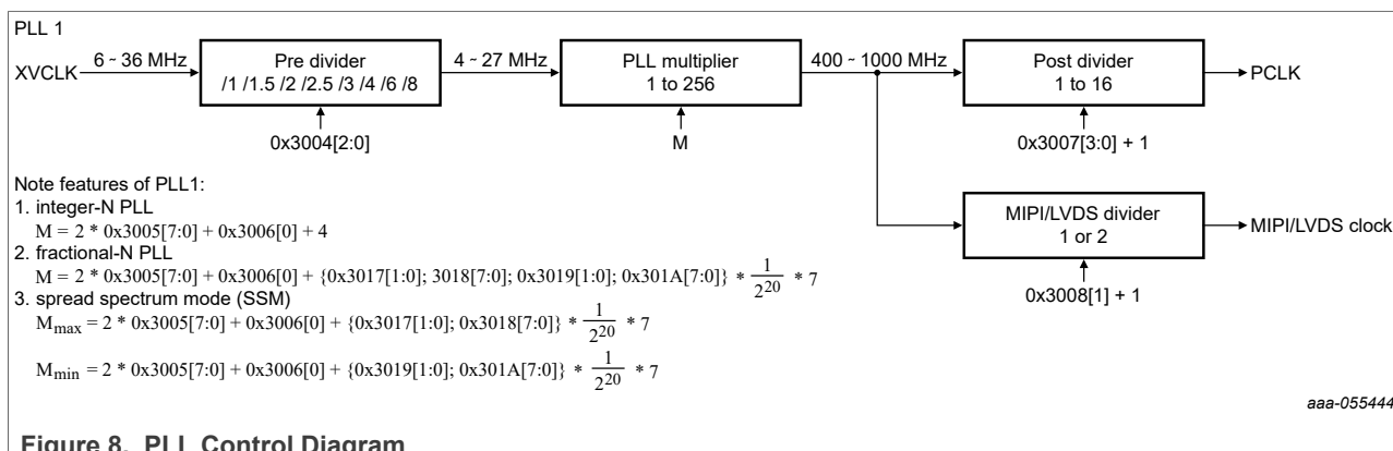
Figure 8. PLL Control Diagram
