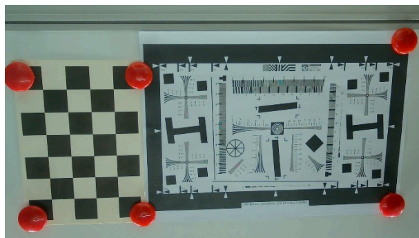
Figure 25. Vertical Flip Off vs. Vertical Flip On
