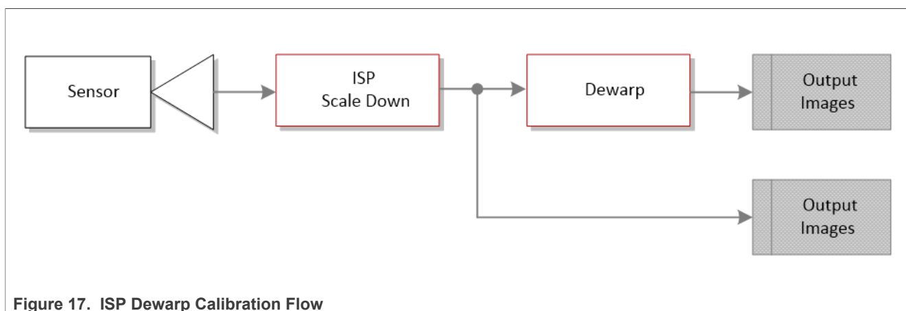
Figure 17. ISP Dewarp Calibration Flow
