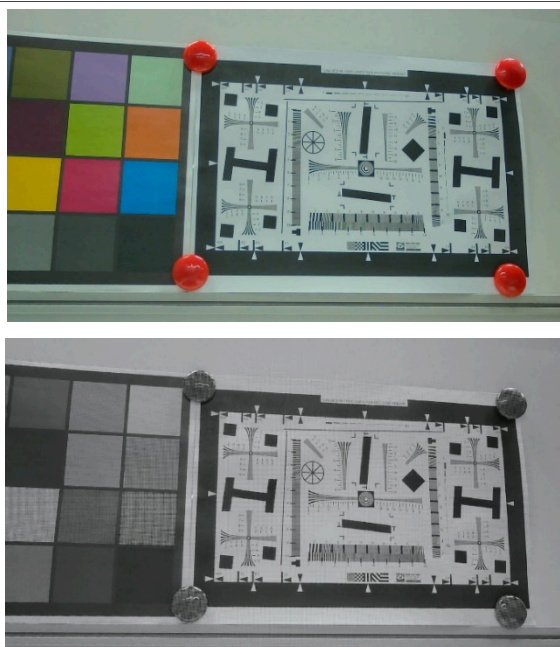
Figure 56. DEMOSAIC ENABLE and BYPASS
