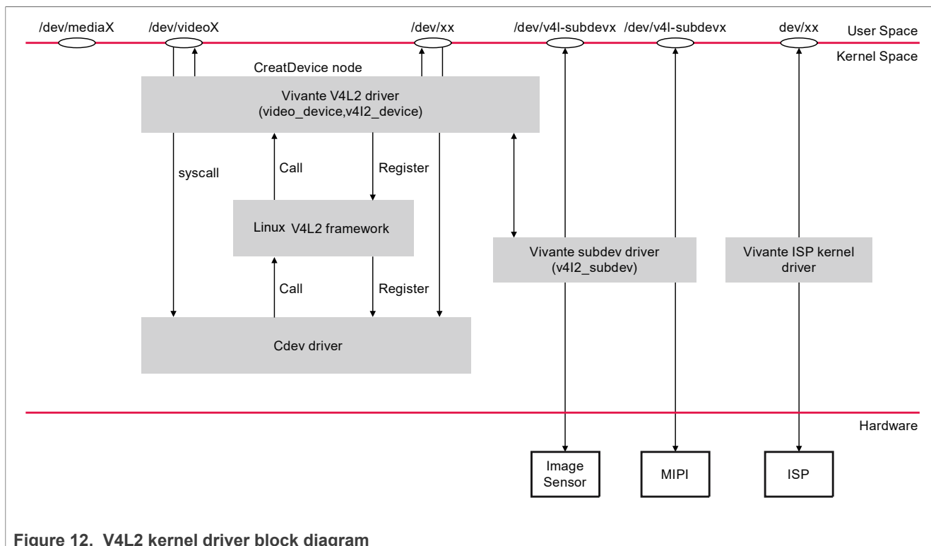
Figure 12. V4L2 kernel driver block diagram
