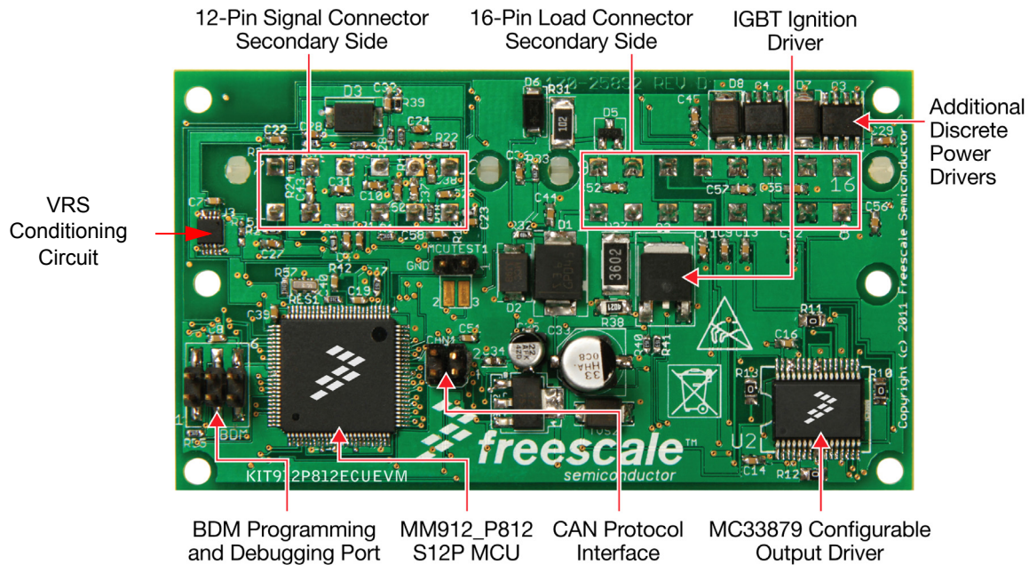
Figure 2. ECU Included in KIT912P812ECUEVM
