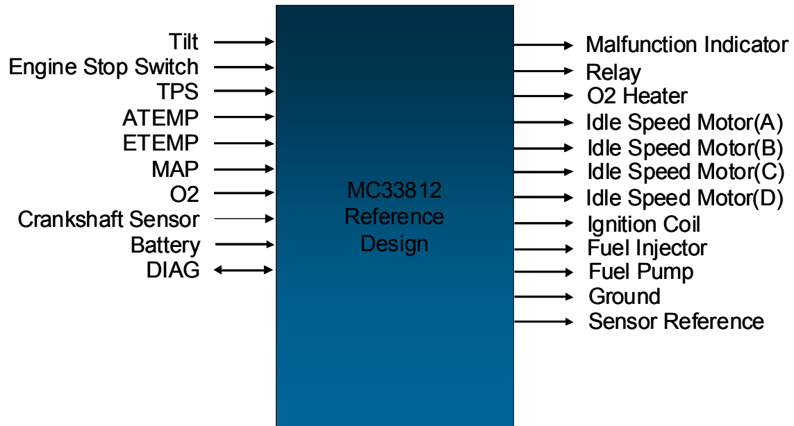
Figure 22. Signals Diagram for the KIT912P812ECUEVM Small Engine Reference Design
