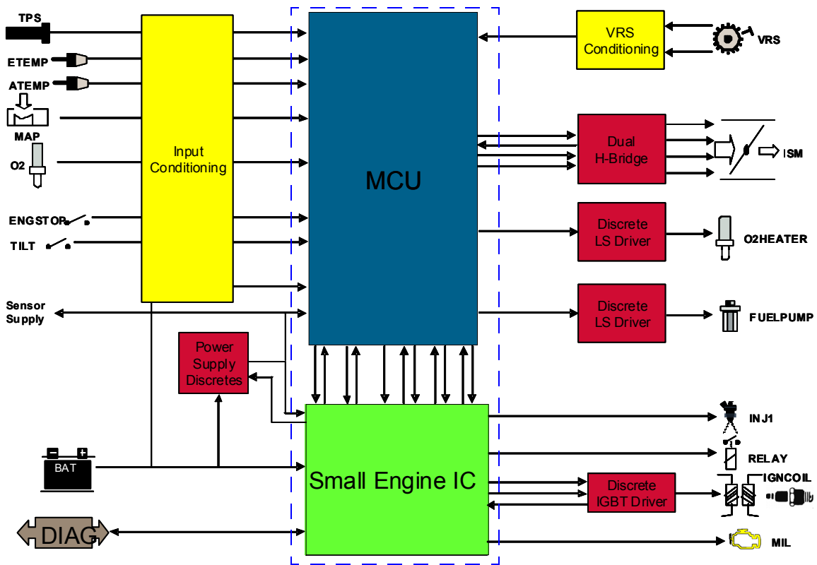
Figure 23. System Block Diagram of KIT912P812ECUEVM and Example System Loads
