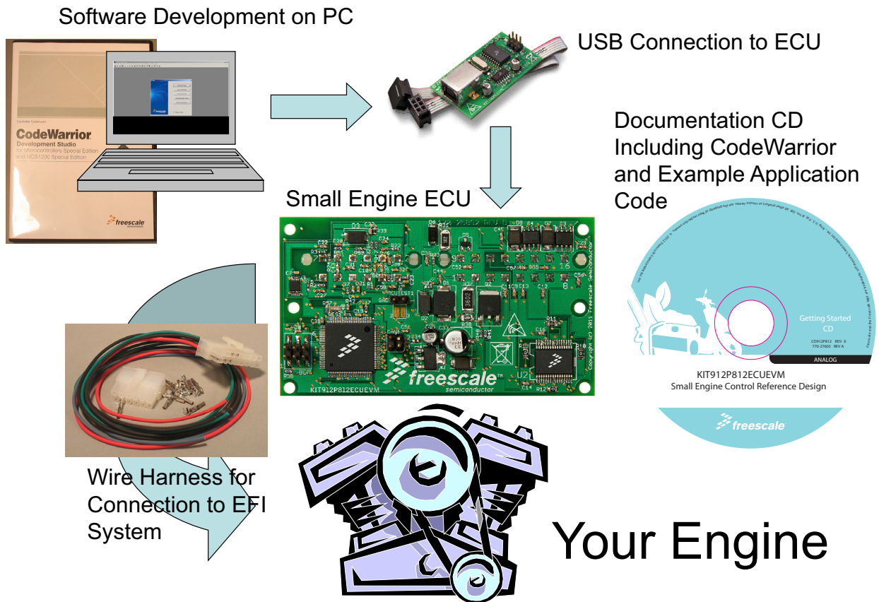
Figure 7. KIT912P812ECUEVM Board Setup
