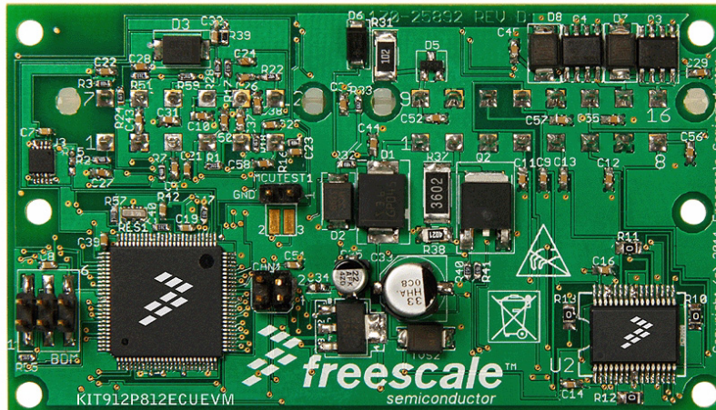
Figure 1. KIT912P812ECUEVM Reference Design Board
