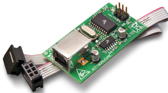
Figure 6. Example USB BDM Tool for Connection to PC
