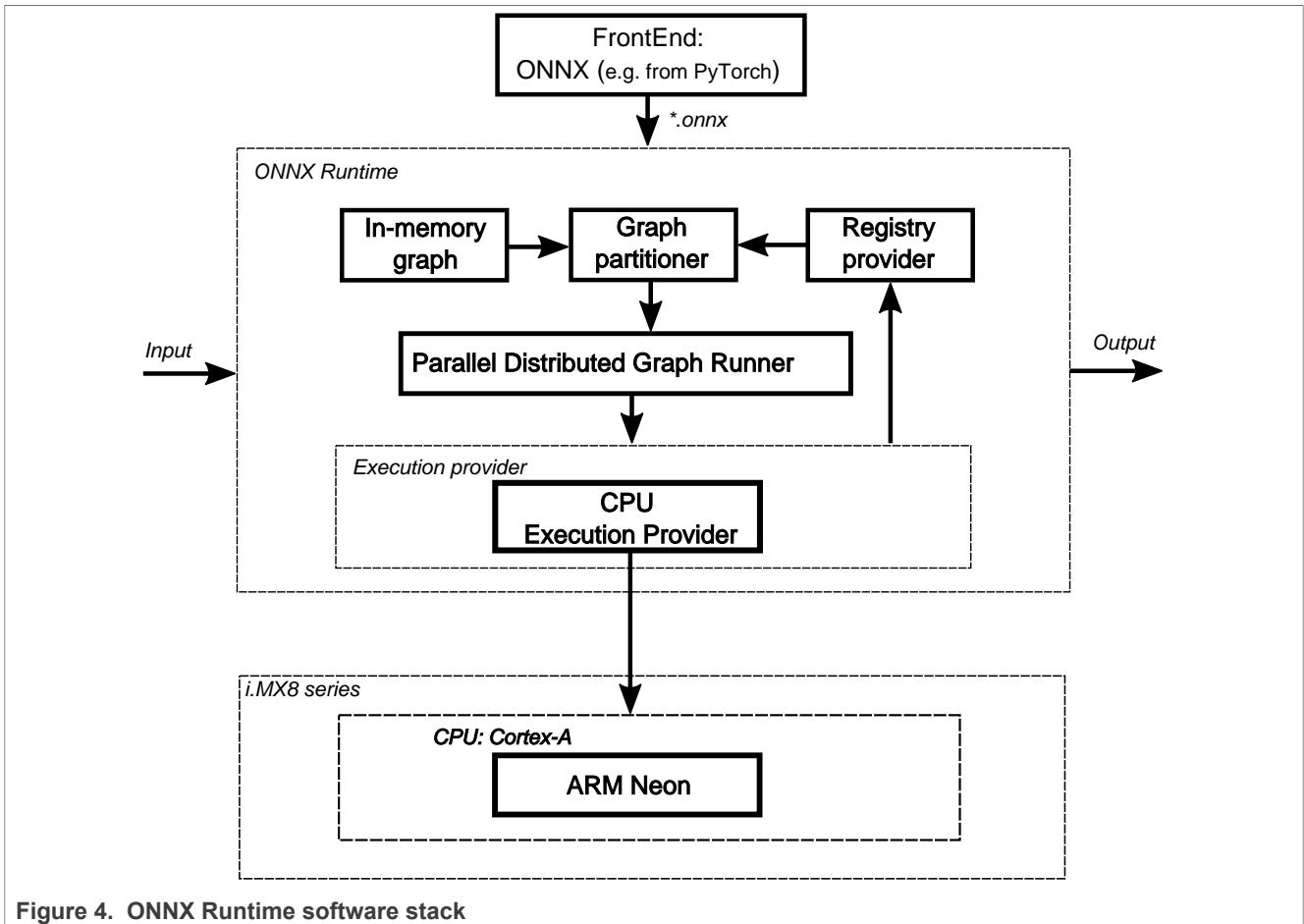
Figure 4. ONNX Runtime software stack
