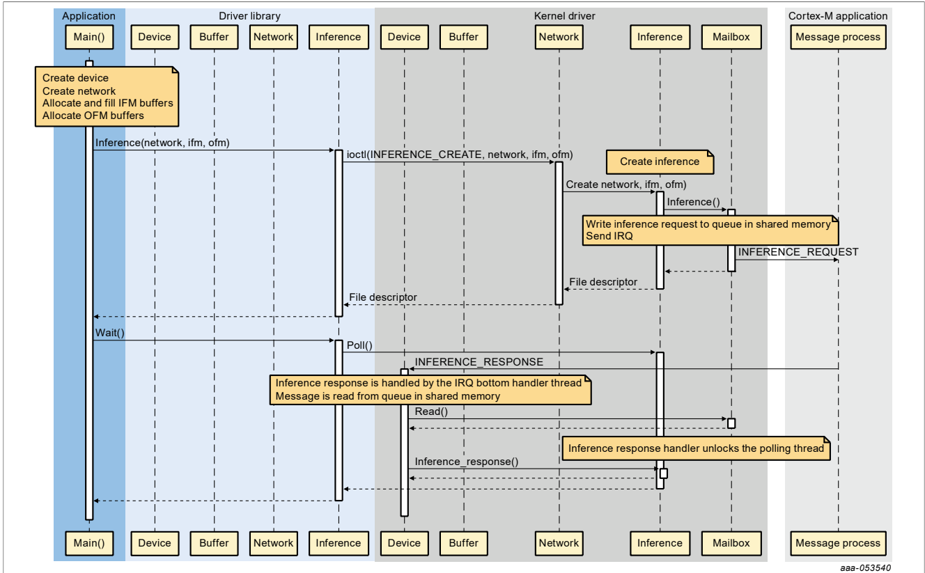
Figure 14. Inference class
