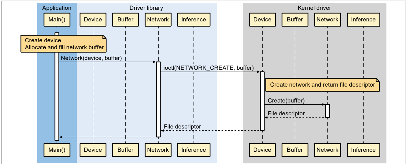
Figure 13. Network class
