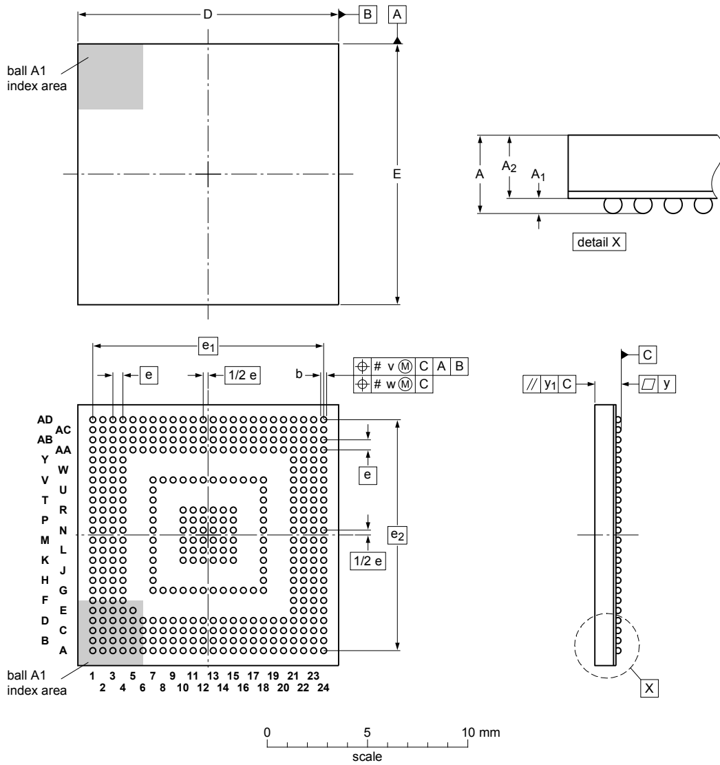
LFBGA401: plastic low profile fine-pitch ball grid array package; 401 balls; body 13 x 13 x 1 mm SOT989-1
