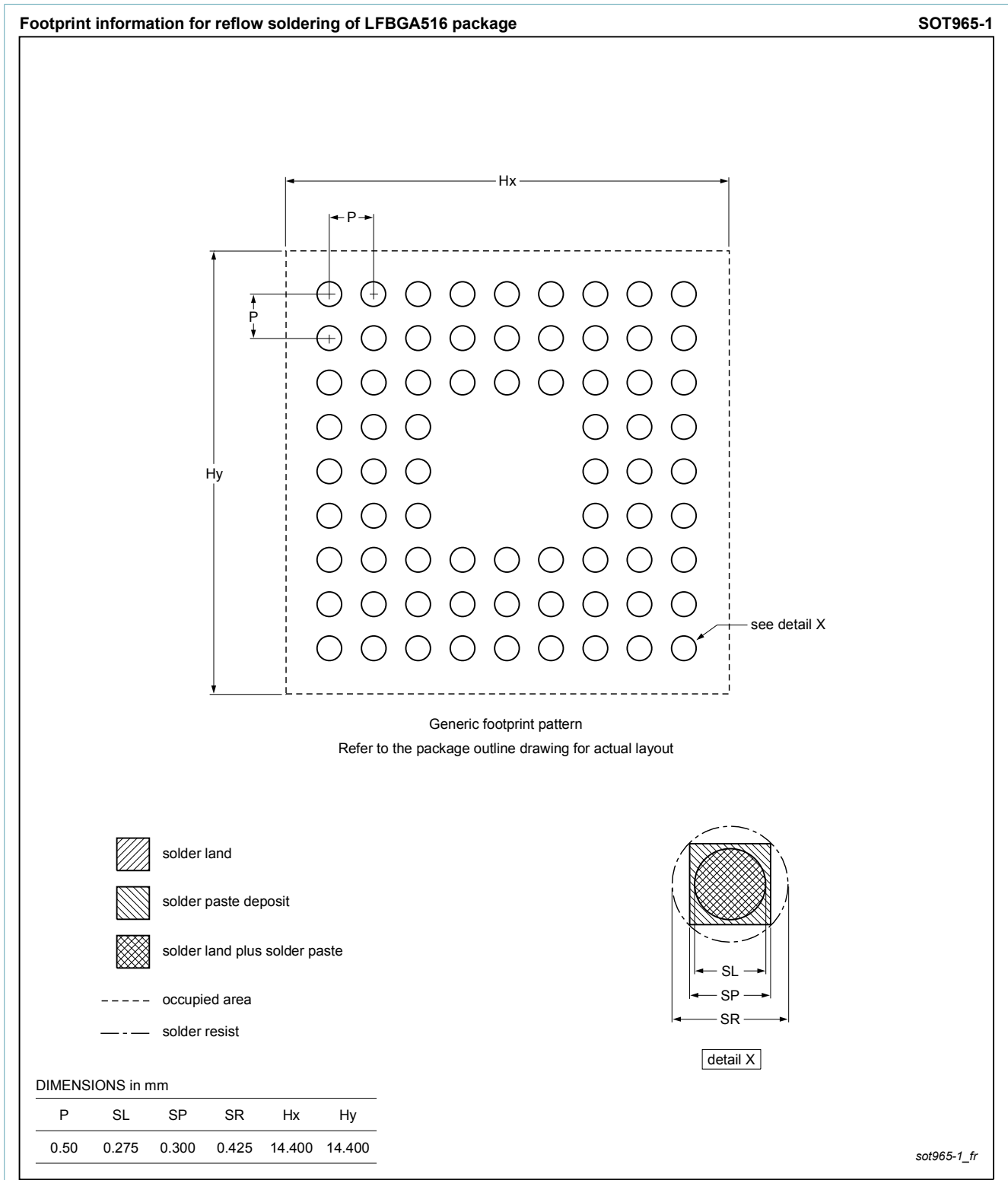
Fig. 2. Reflow soldering footprint for LFBGA516 (SOT965-1)
