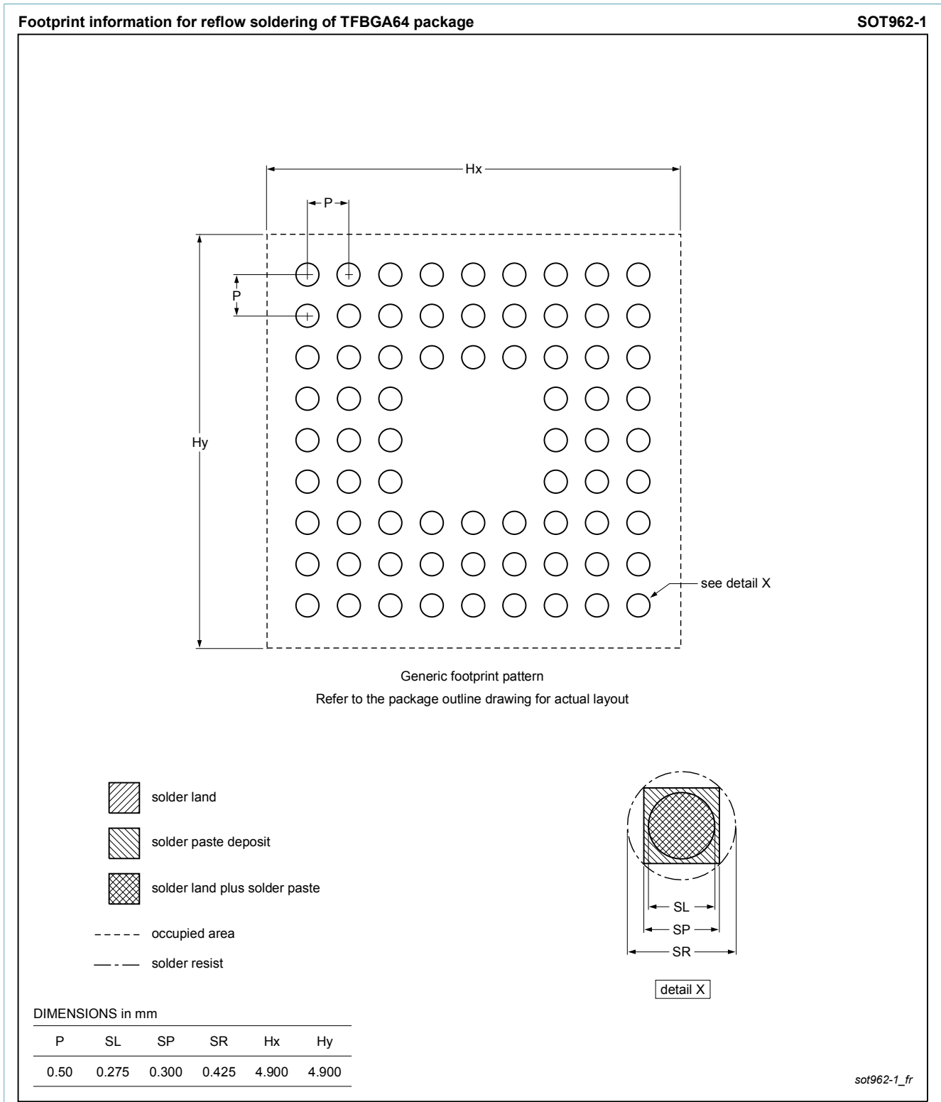
Fig. 2. Reflow soldering footprint for TFBGA64 (SOT962-1)
