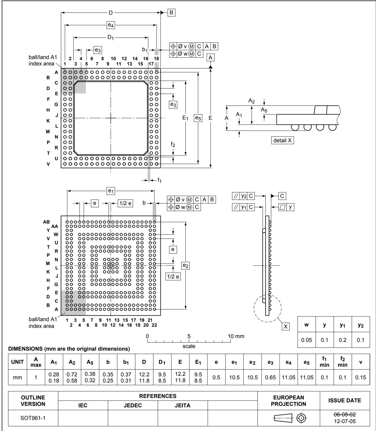
Fig. 1. Package outline VFBGA352S (SOT961-1)
