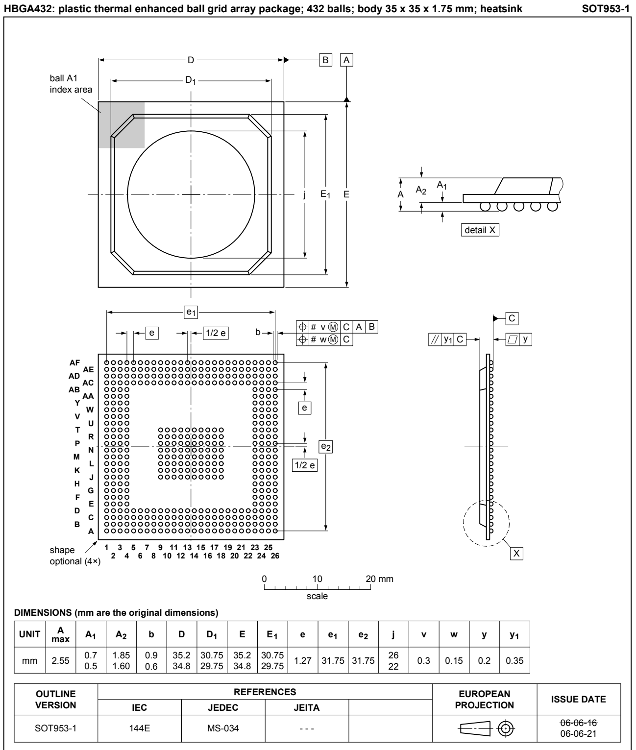
Fig. 1. Package outline HBGA432 (SOT953-1)
