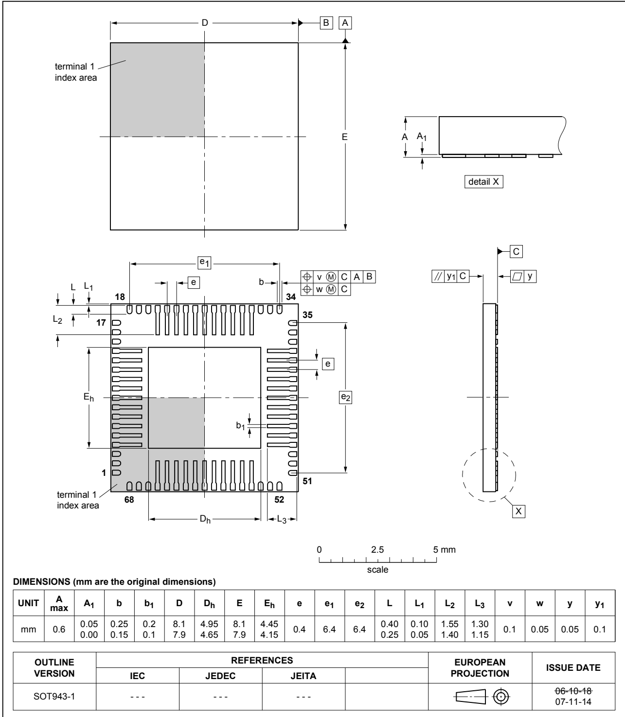
Fig. 1. Package outline HUQFN68U (SOT943-1)
