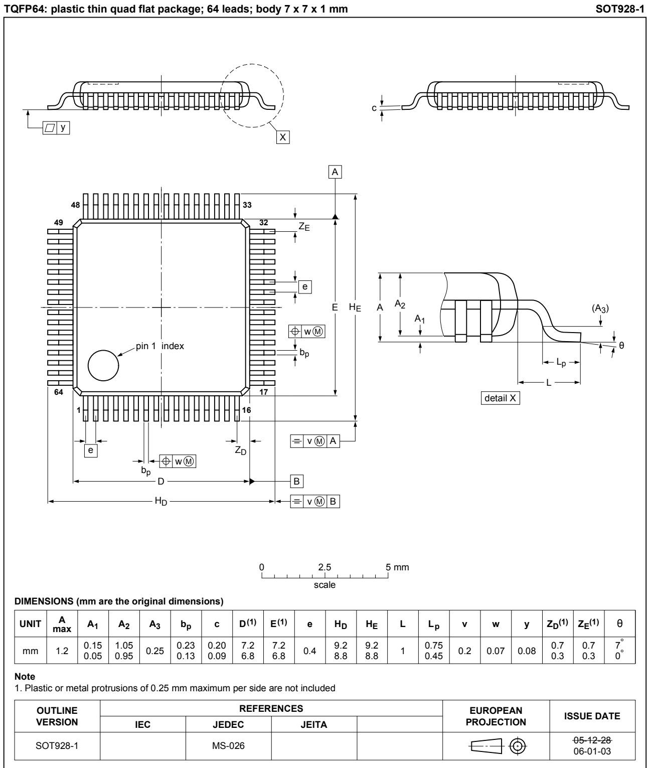
Fig. 1. Package outline TQFP64 (SOT928-1)
