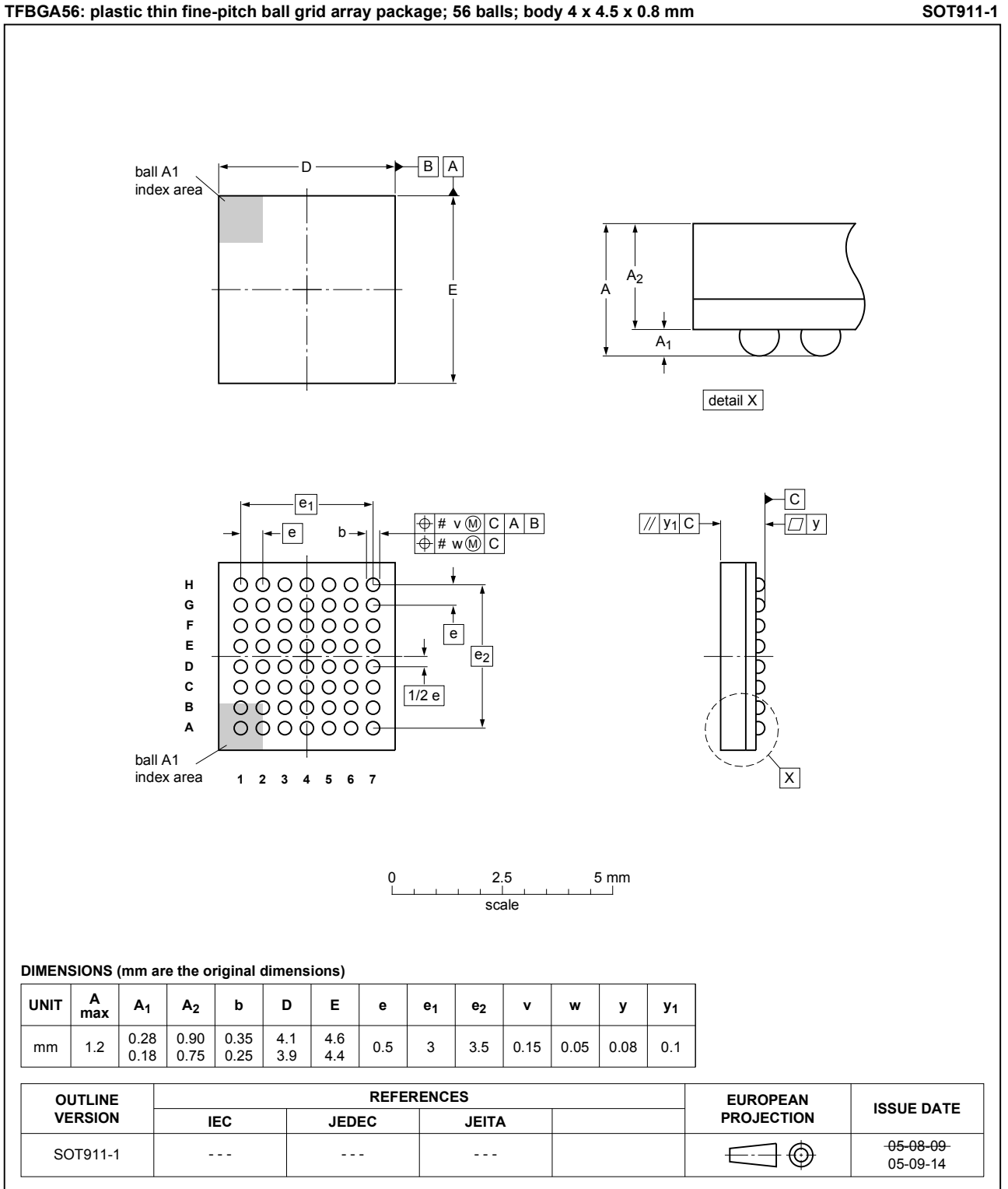
Fig. 1. Package outline TFBGA56 (SOT911-1)
