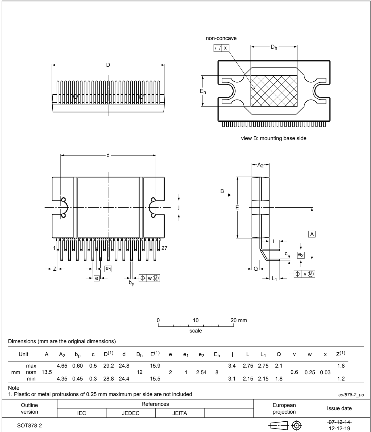
Fig. 1. Package outline RDBS27P (SOT878-2)
