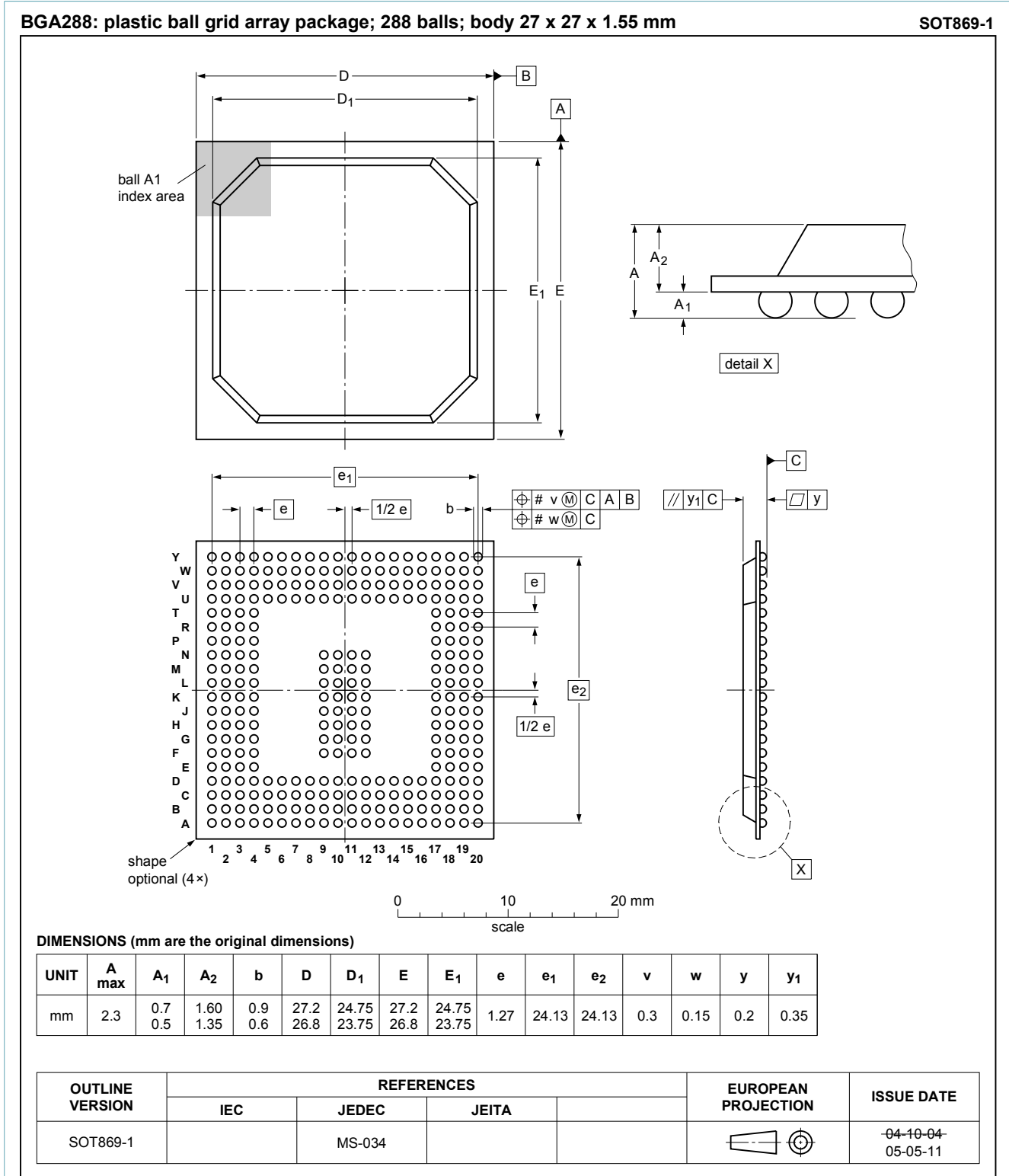
Fig. 1. Package outline BGA288 (SOT869-1)
