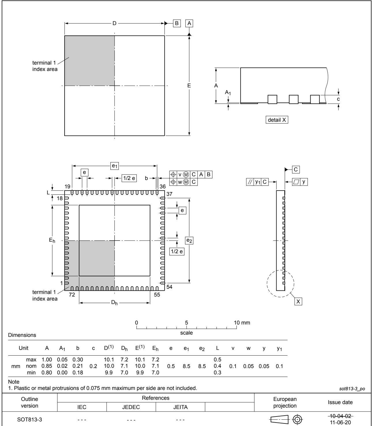
Fig. 1. Package outline HVQFN72 (SOT813-3)
