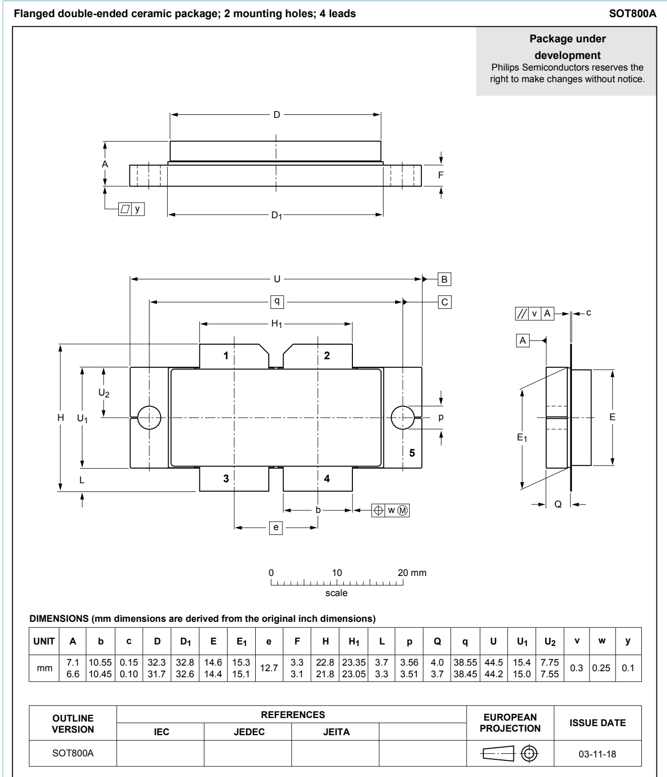
Fig. 1. Package outline SOT800A
