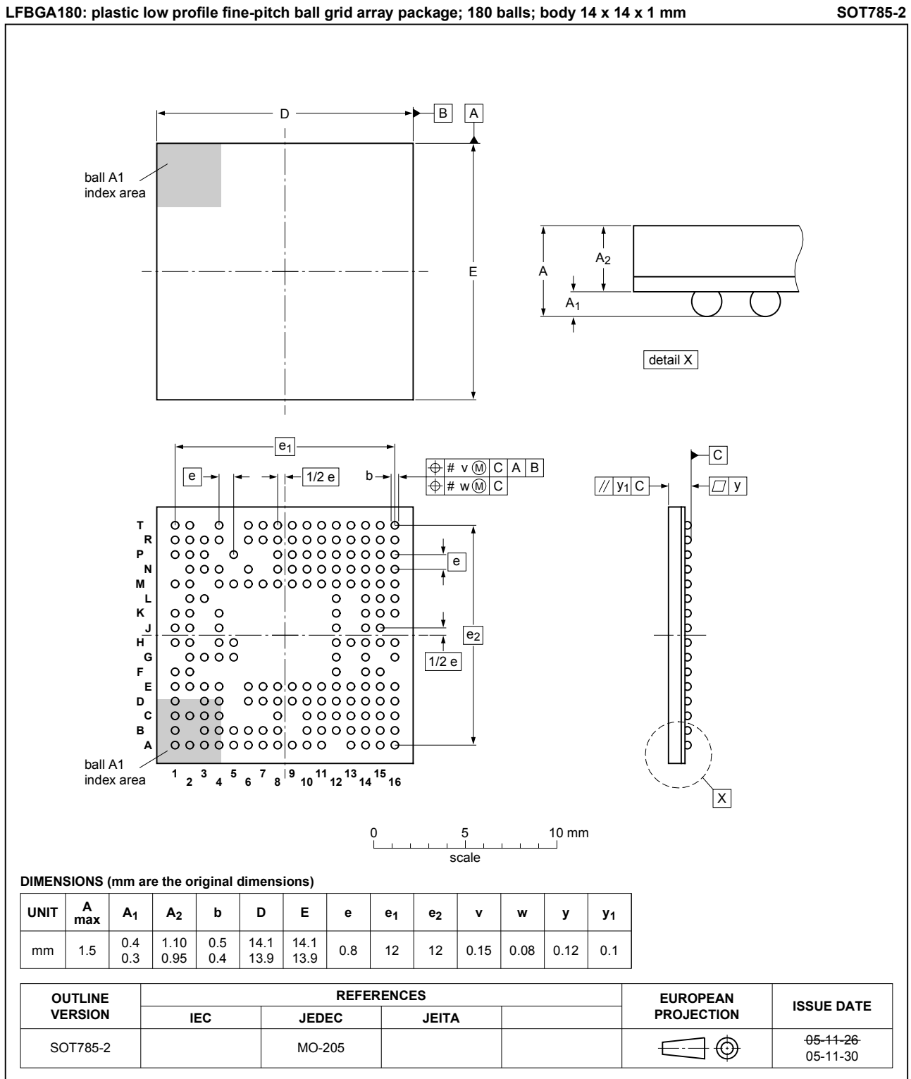
Fig. 1. Package outline LFBGA180 (SOT785-2)
