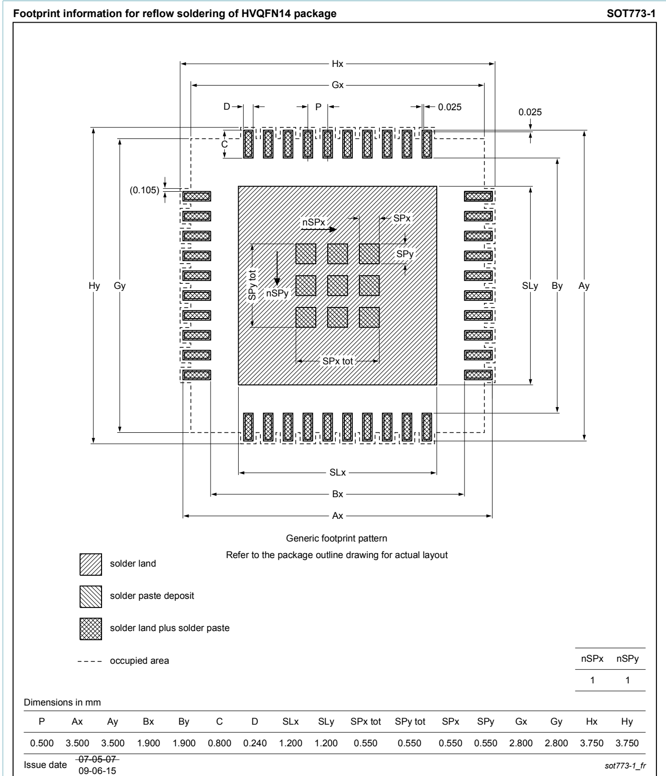
Fig. 2. Reflow soldering footprint for HVQFN14 (SOT773-1)
