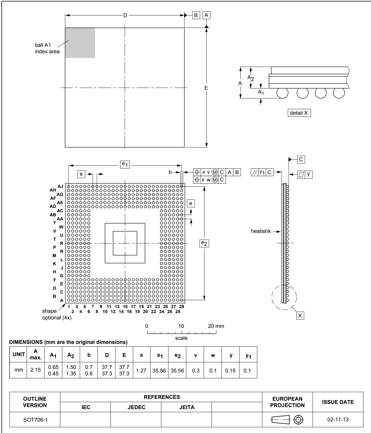
Fig. 1. Package outline HBGA552 (SOT706-1)
