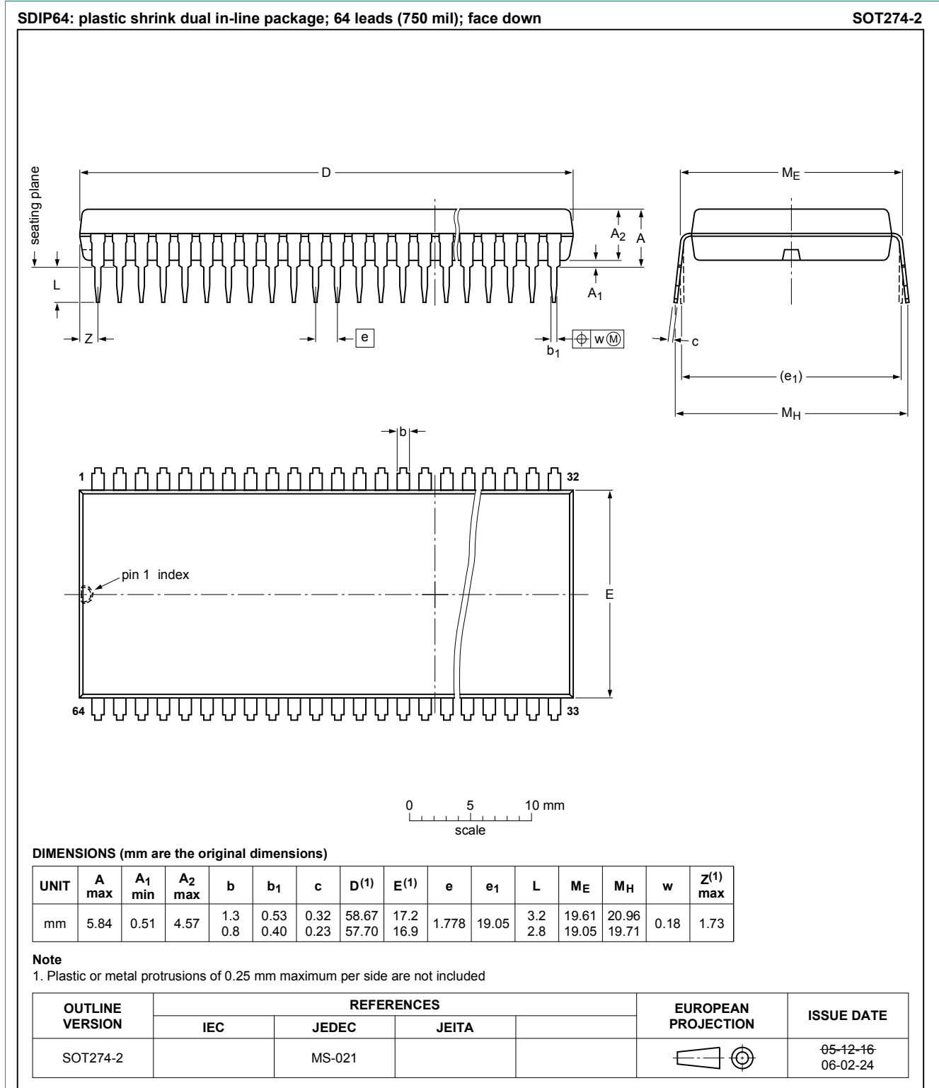
Figure 1. Package outline SDIP64 (SOT274-2)
