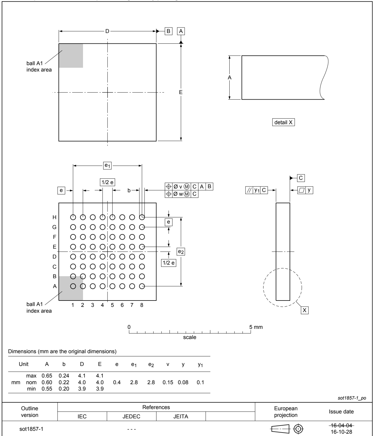
Fig. 1. Package outline UFLGA (SOT1857-1)
