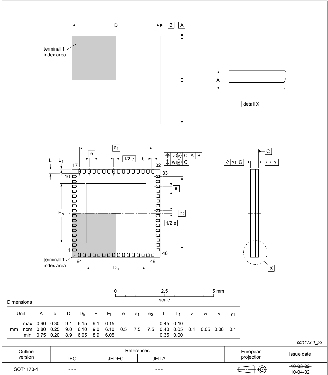
Fig. 1. Package outline HVQFN64R (SOT1173-1)
