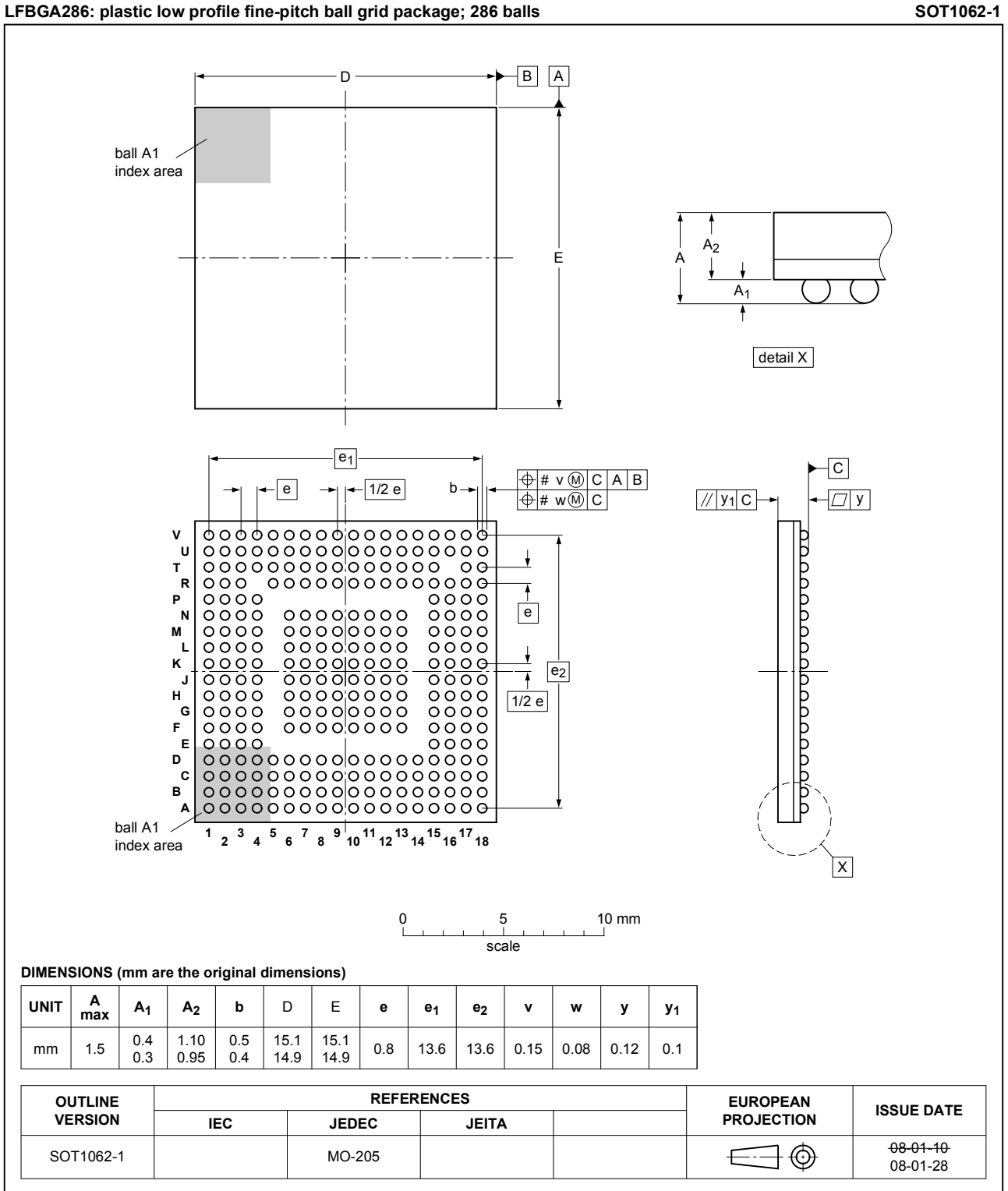
Fig. 1. Package outline LFBGA286 (SOT1062-1)
