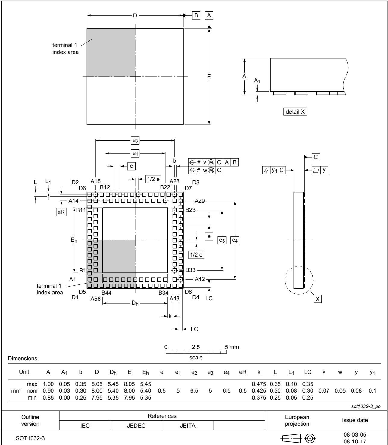
Fig. 1. Package outline HVQFN108U (SOT1032-3)
