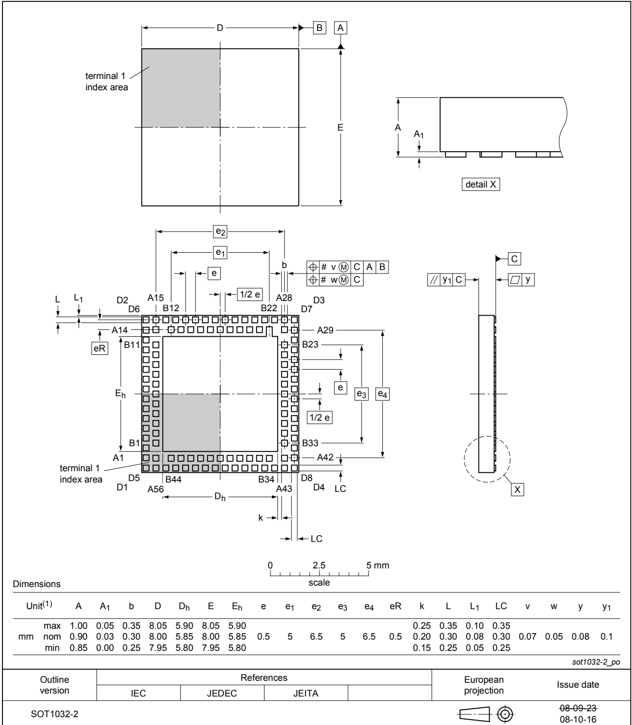
Fig. 1. Package outline HVQFN108U (SOT1032-2)
