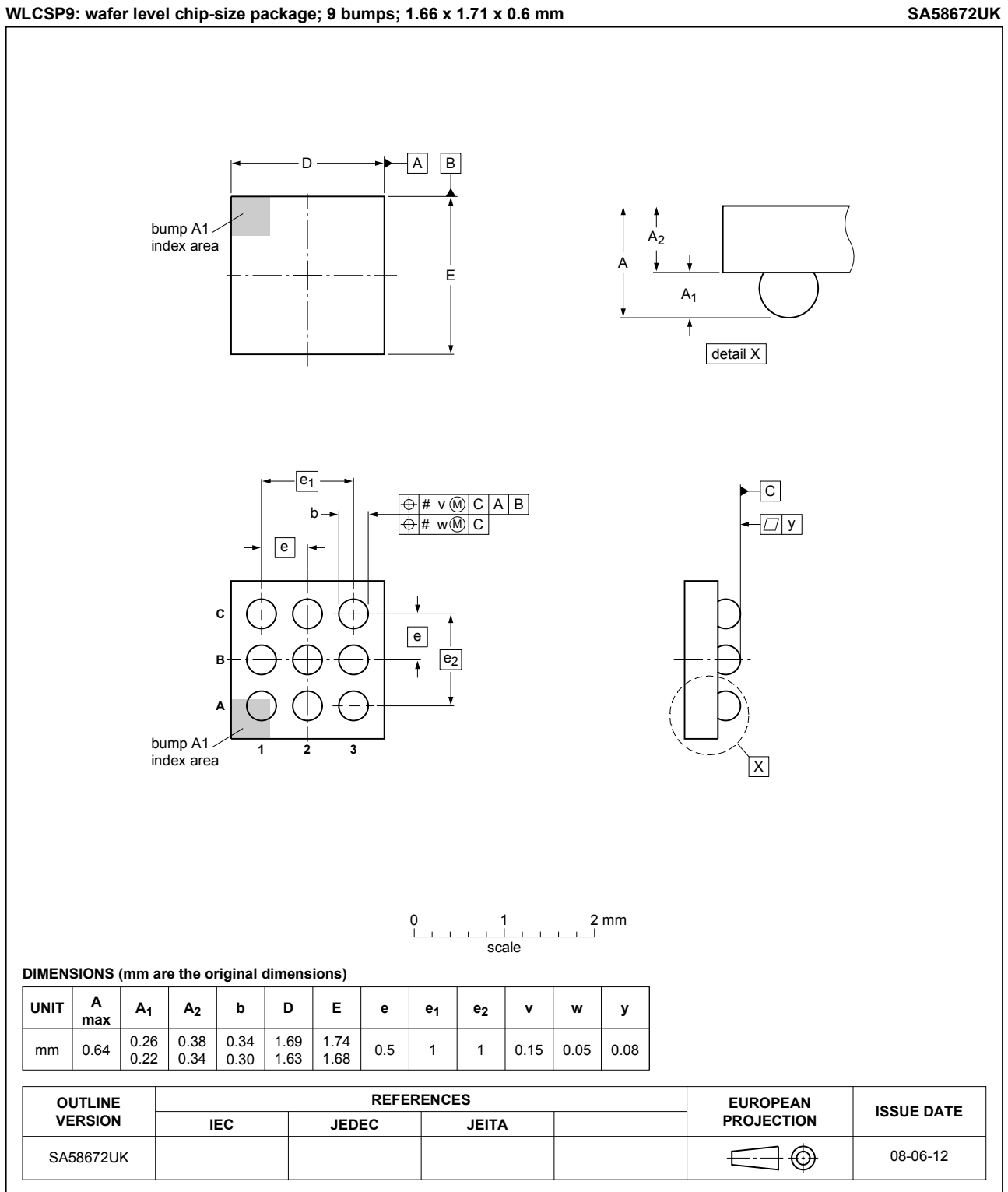
Fig. 1. Package outline WLCSP (OL-SA58672UK)
