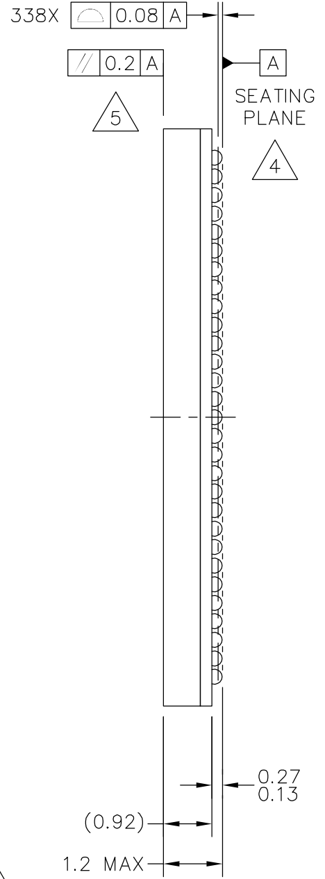
SIDE VIEW
