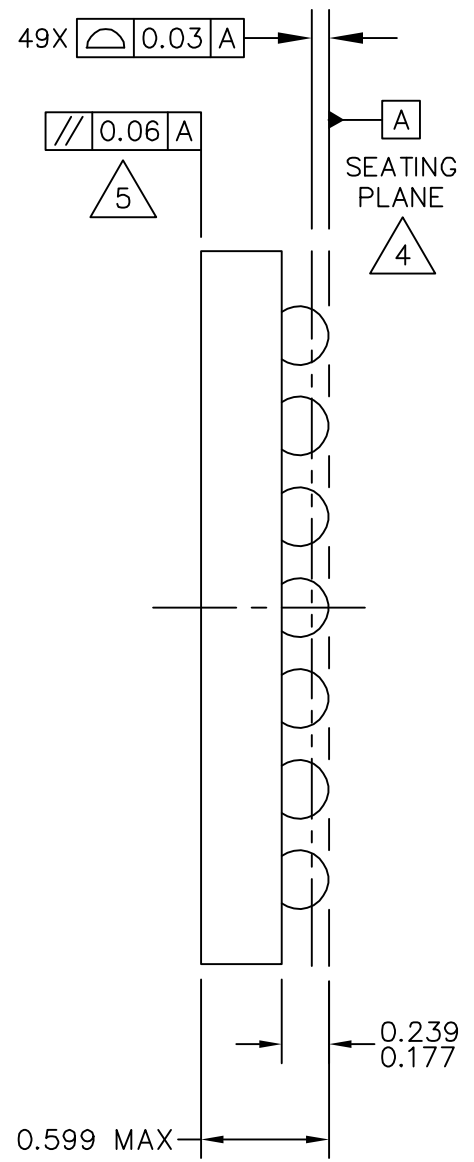
VIEW D-D
