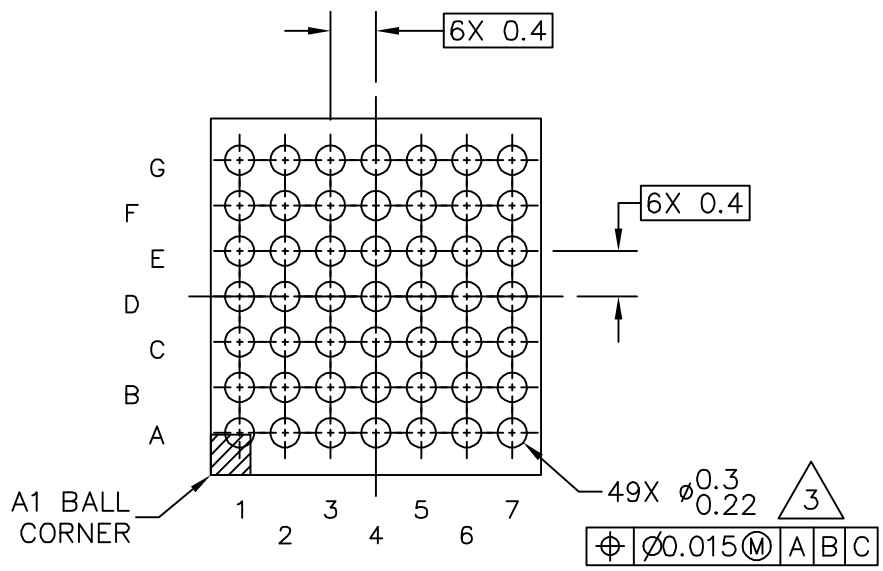
BOTTOM VIEW
