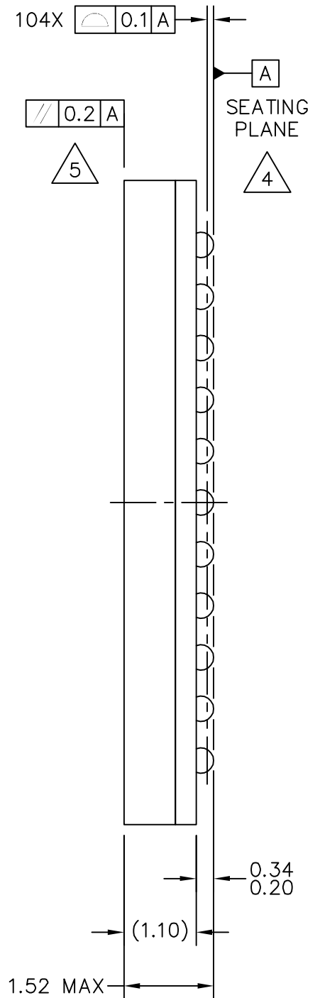
SIDE VIEW
