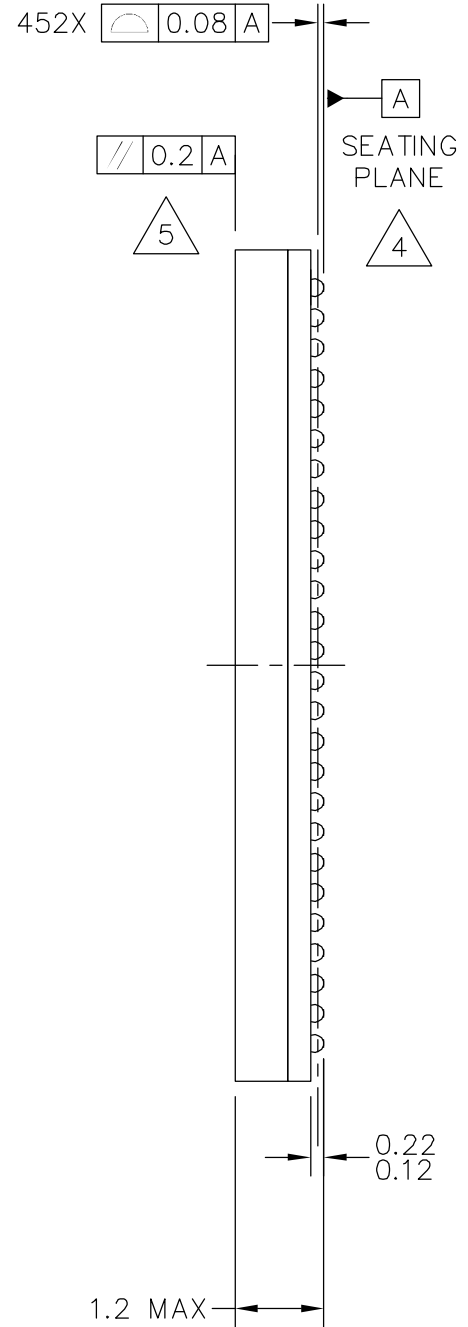
SIDE VIEW
