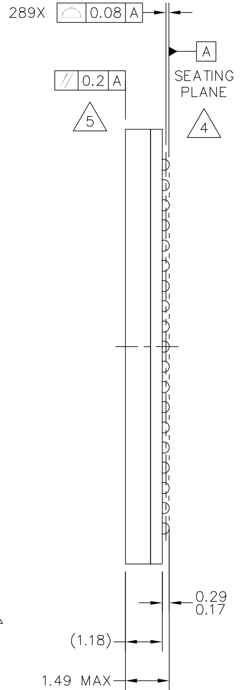
SIDE VIEW
