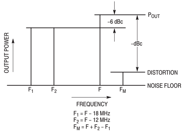
Figure 25. Frequency — Power Relationships for DIN45004B
