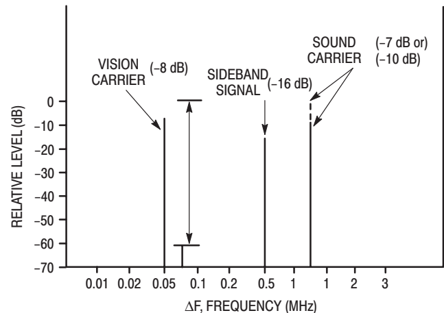
Figure 26. 3rd Order IMD Test for TV
