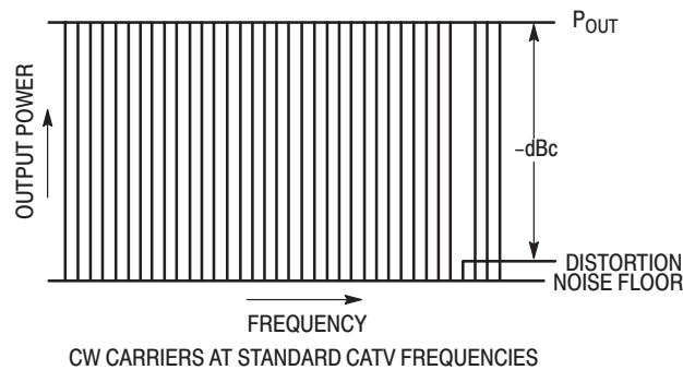
Figure 24. Frequency — Power Relationships for CTB
