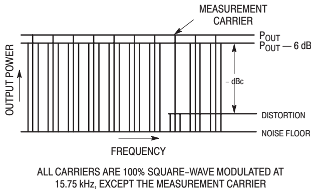
Figure 23. Frequency — Power Relationships for XMD
