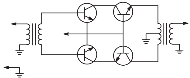
Figure 19. Basic CATV Amplifier
