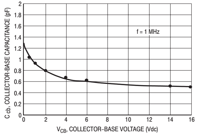
Figure 4. Junction Capacitance versus Voltage
