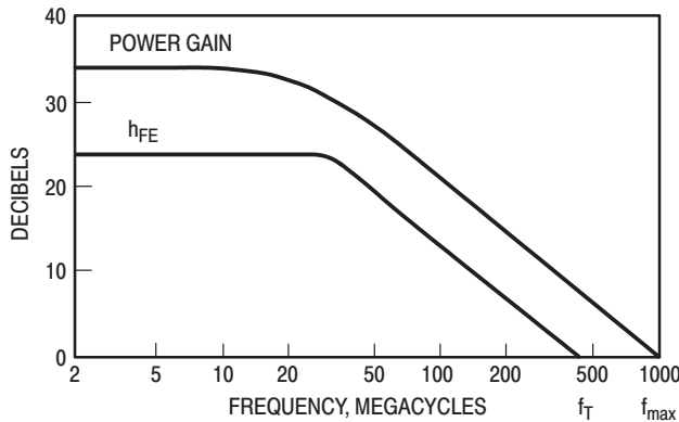
Figure 3. Beta versus Frequency
