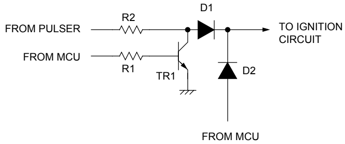
Figure 5. Analog Ignition Control
