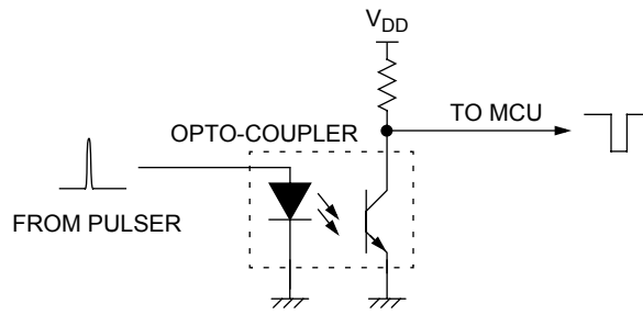
Figure 7. Pulse Shaping
