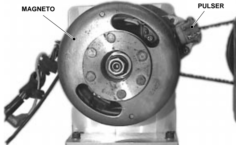
Figure 1. Magneto/Pulser Assembly
