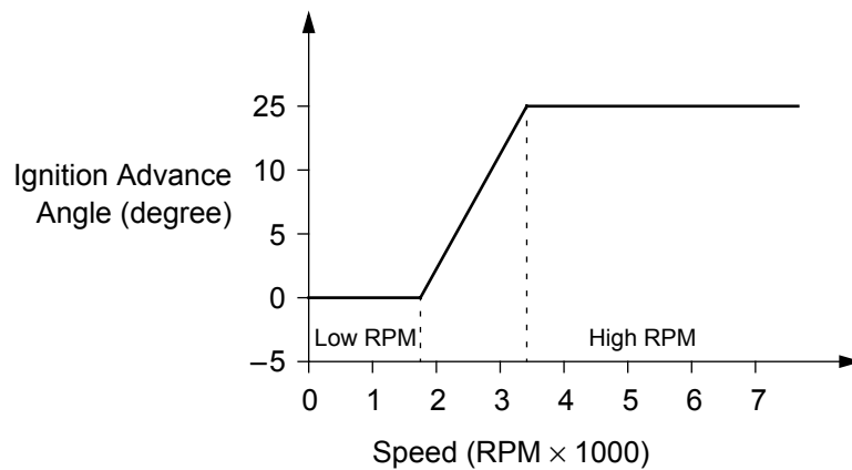
Figure 9. Ignition Advance Characteristics
