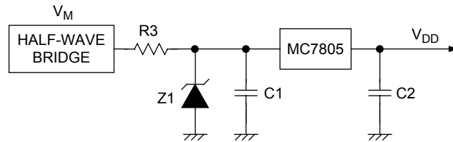
Figure 6. DC Power Supply
