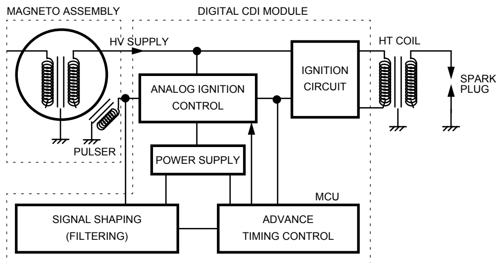
Figure 4. Typical Digital CDI System Block Diagram
