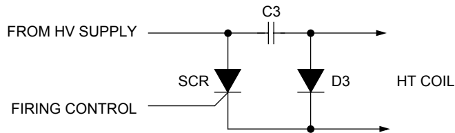
Figure 8. Advance Timing Control
