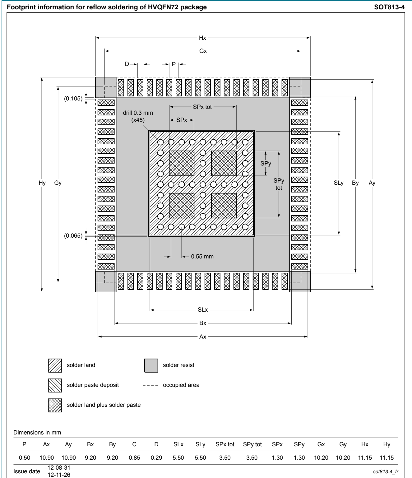
Figure 2. Reflow soldering footprint for HVQFN72 (SOT813-4)
