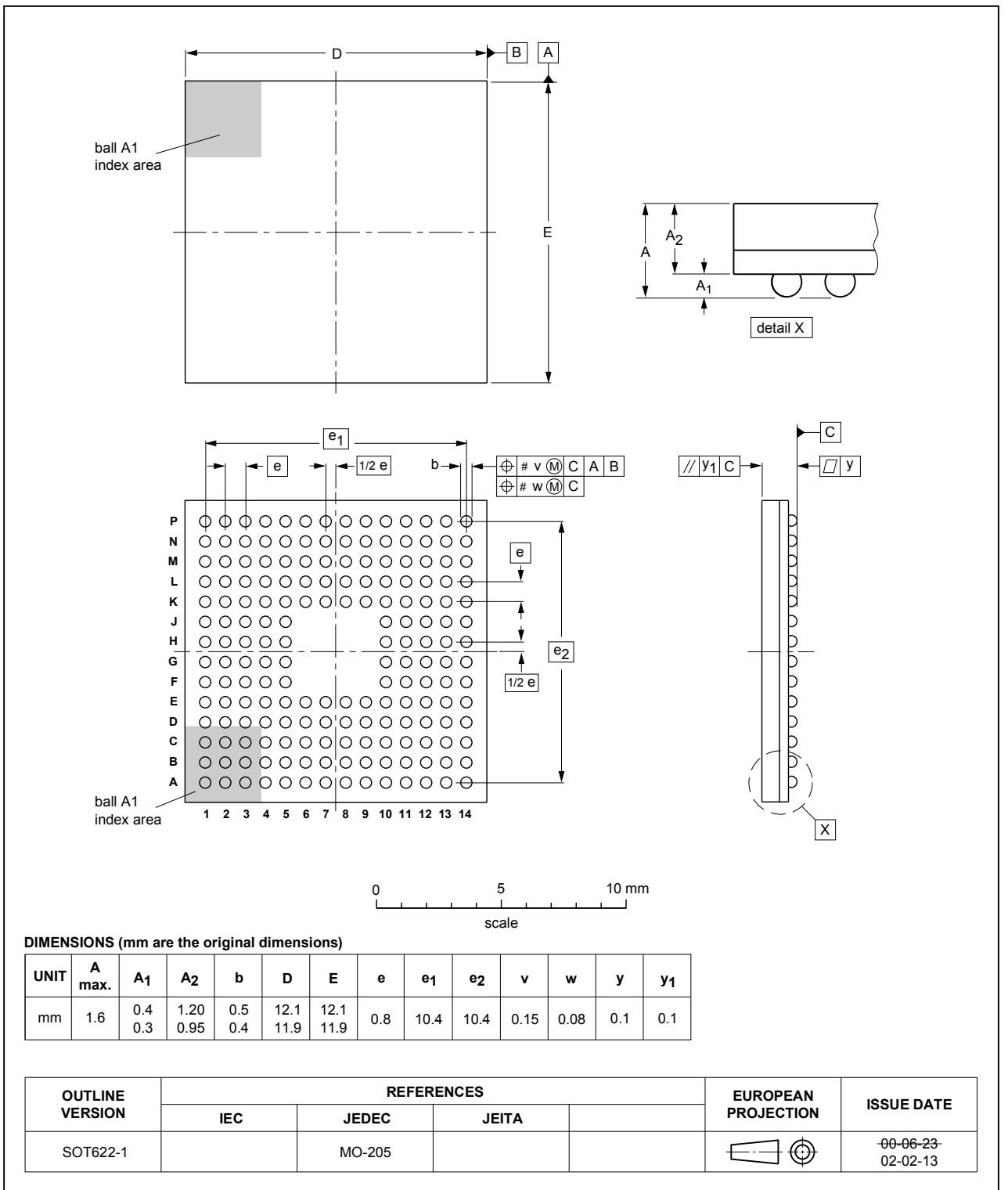
Fig. 1. Package outline LFBGA180 (SOT622-1)
