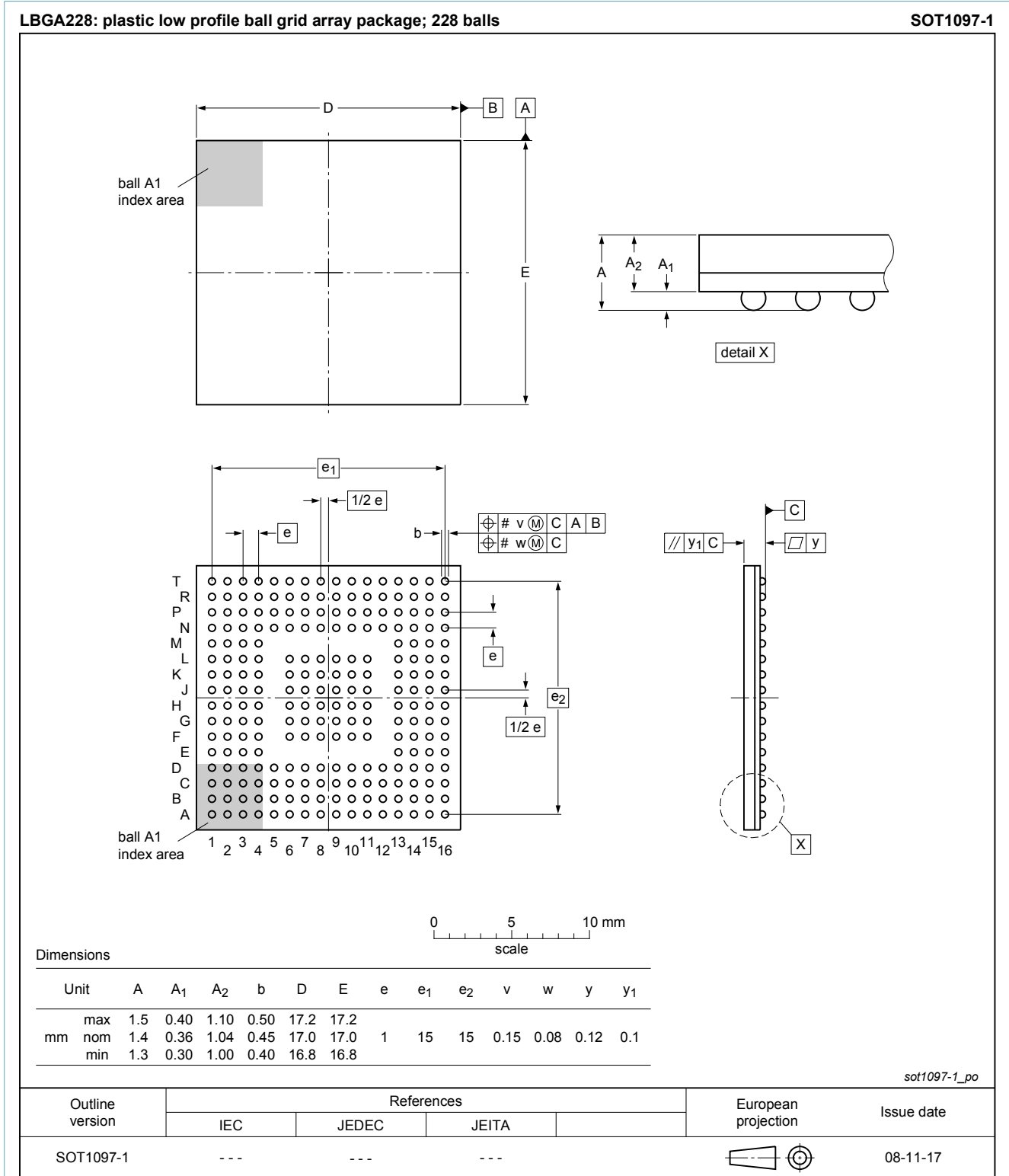
Fig. 1. Package outline LPGA228 (SOT1097-1)
