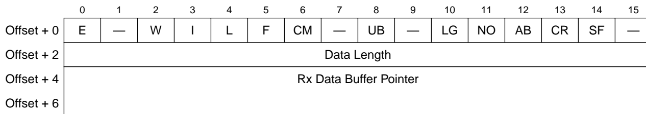
Figure 11-9. SS7 Receive Buffer Descriptor (RxBD)
