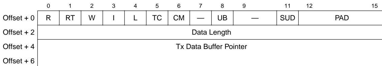
Figure 11-10. SS7 Transmit Buffer Descriptor (TxBD)
