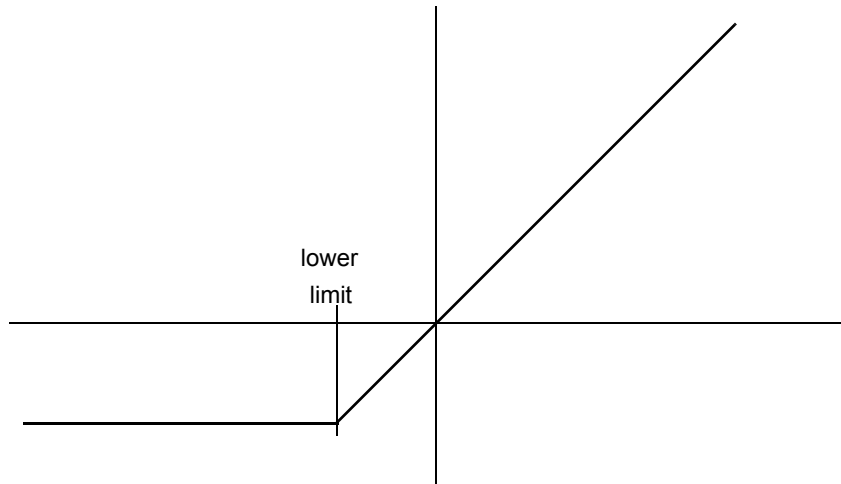
Figure 3-13. Algorithm Transition
