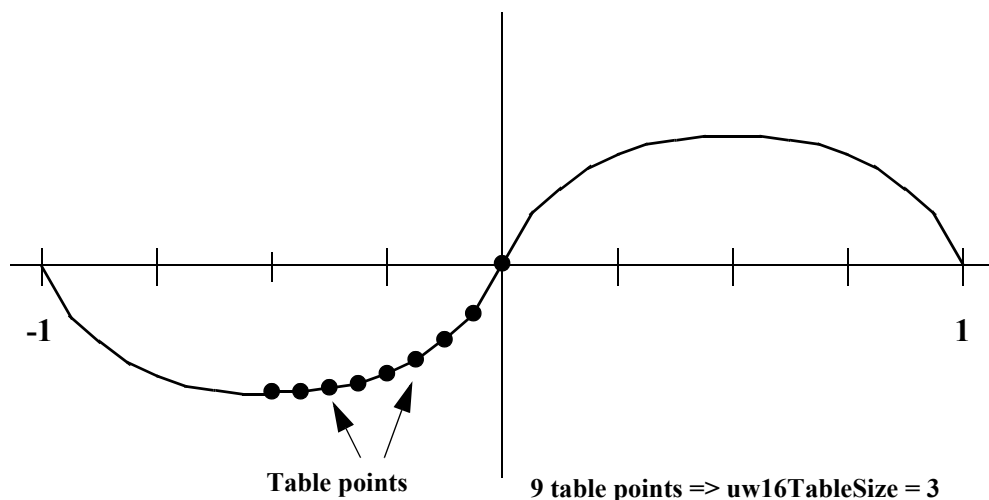
Figure 3-1. Algorithm Diagram
