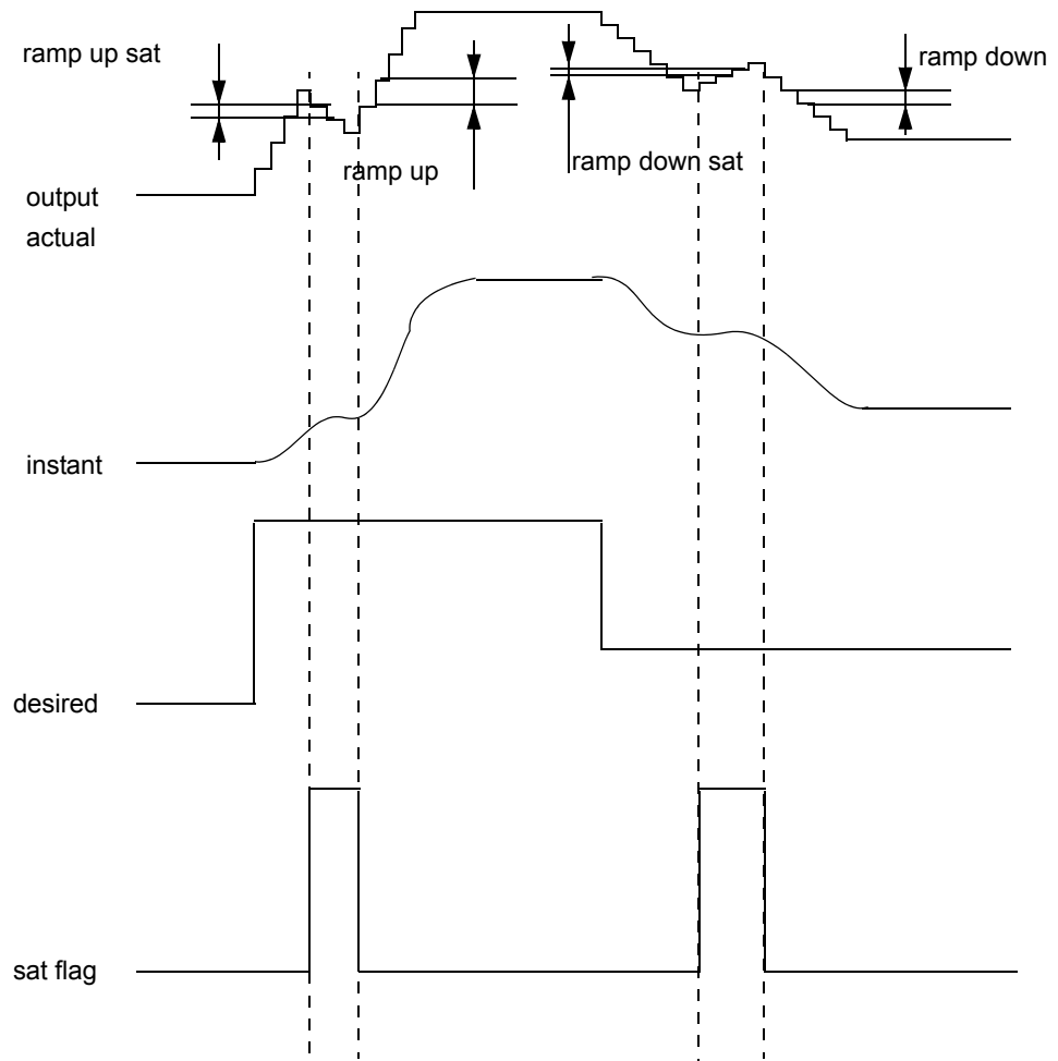
Figure 3-11. Algorithm Diagram
