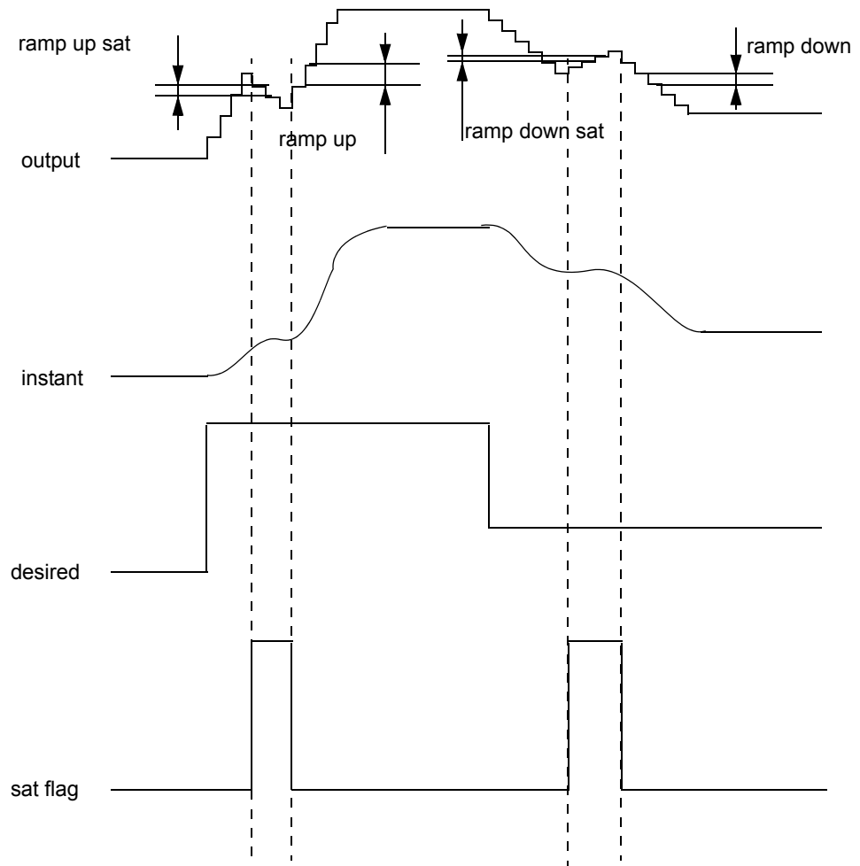
Figure 3-10. Algorithm Diagram
