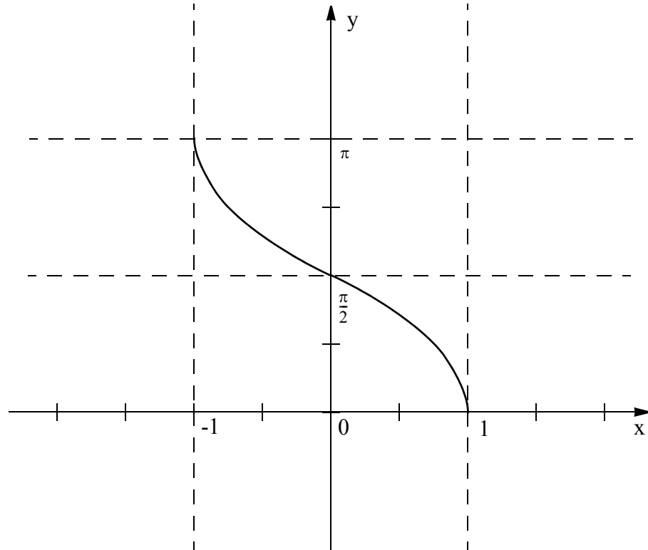
Figure 3-5. GFLIB_Acos Function
