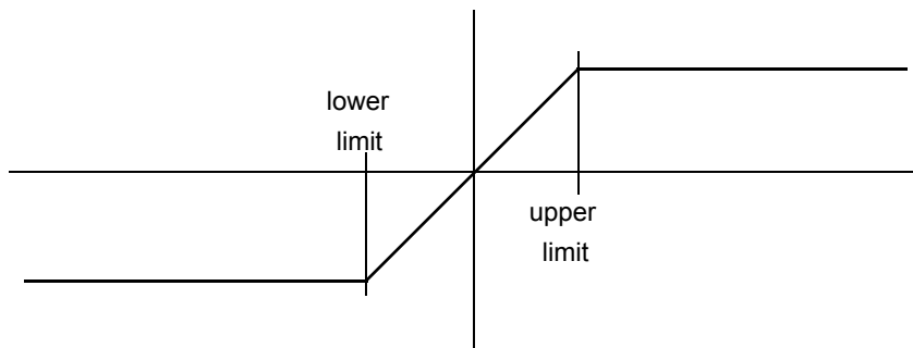
Figure 3-15. Algorithm Transition
