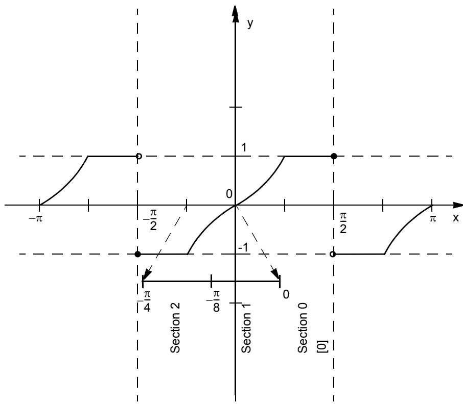
Figure 3-3. GFLIB_Tan Function
