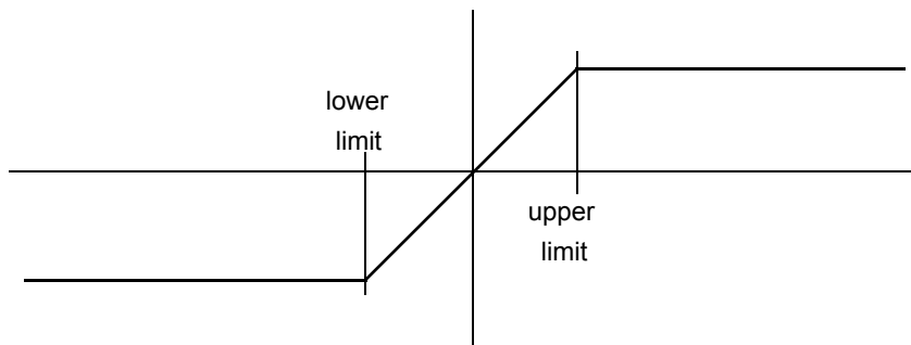
Figure 3-12. Algorithm Transition
