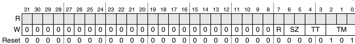
Figure 18-7. BDM Address Attribute Register (BAAR)
