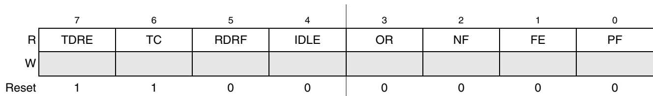
Figure 15-9. SCI Status Register 1 (SC1xS1)
