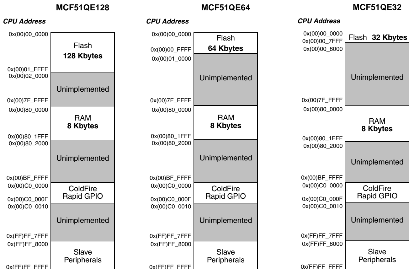
Figure 4-1. MCF51QE128/64/32 Memory Maps
