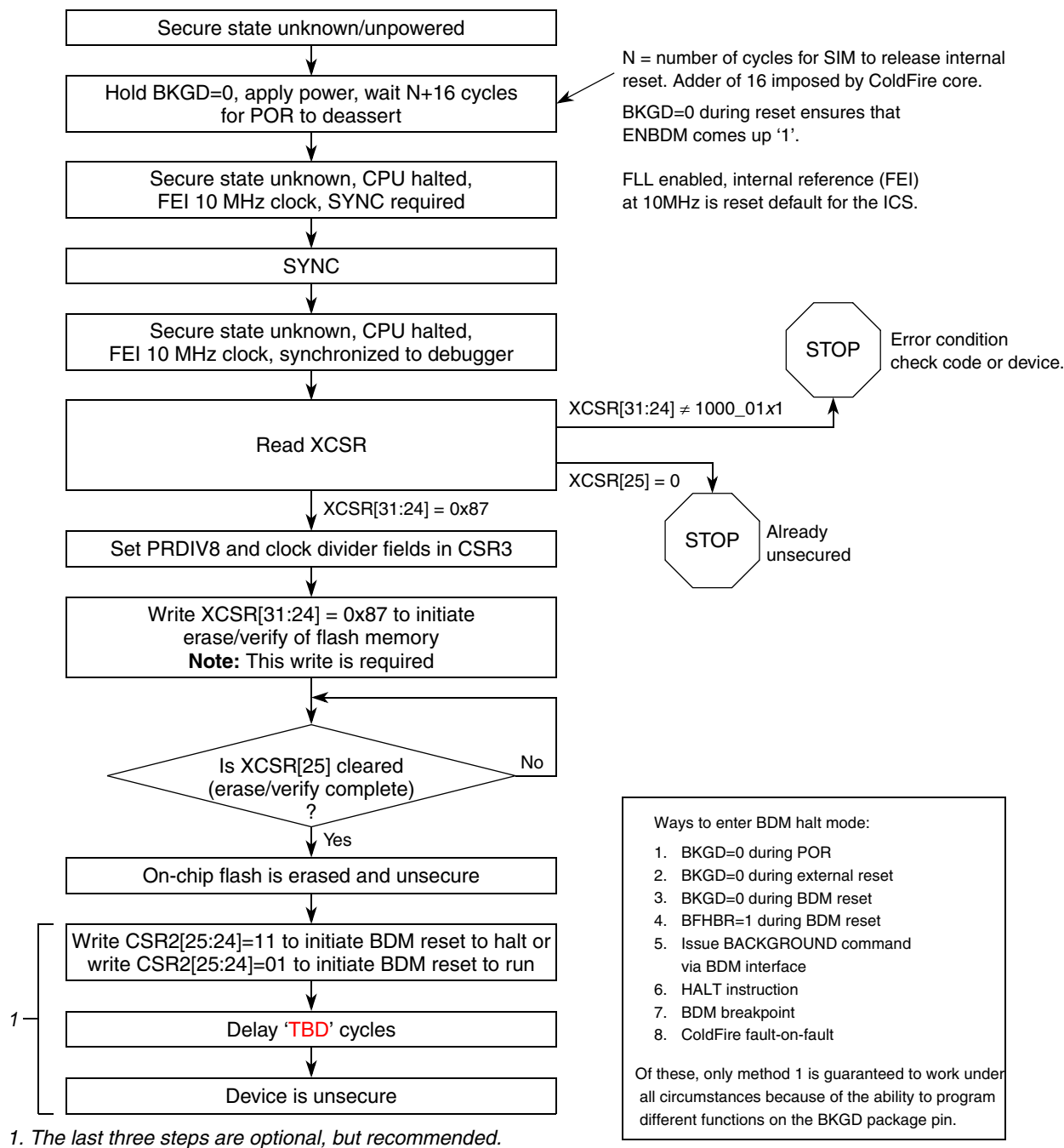
Figure 4-15. Procedure for Clearing Security on MCF51QE128/64/32 via the BDM Port
