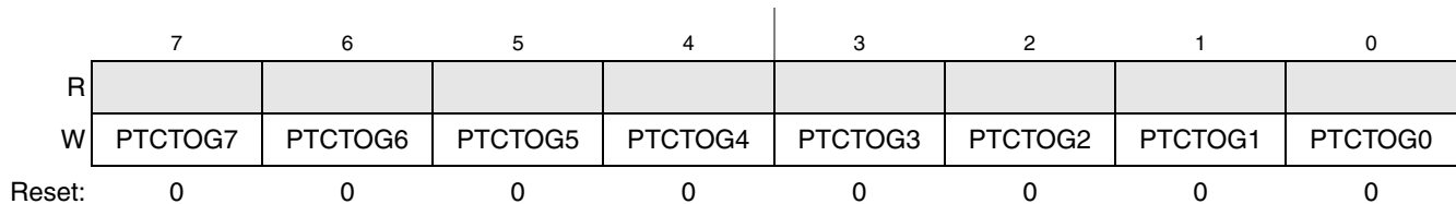
Figure 6-18. Port C Toggle Enable Register (PTCTOG)
