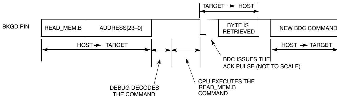
Figure 18-20. Handshake Protocol at Command Level
