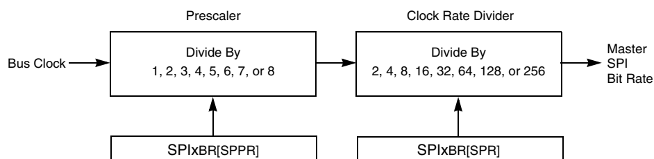
Figure 16-4. SPI Baud Rate Generation
