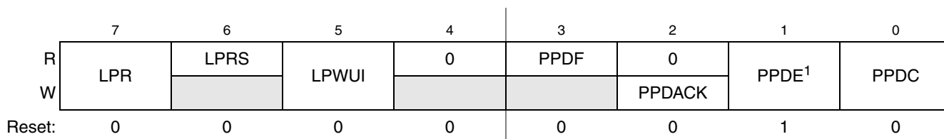
Figure 5-8. System Power Management Status and Control 2 Register (SPMSC2)
