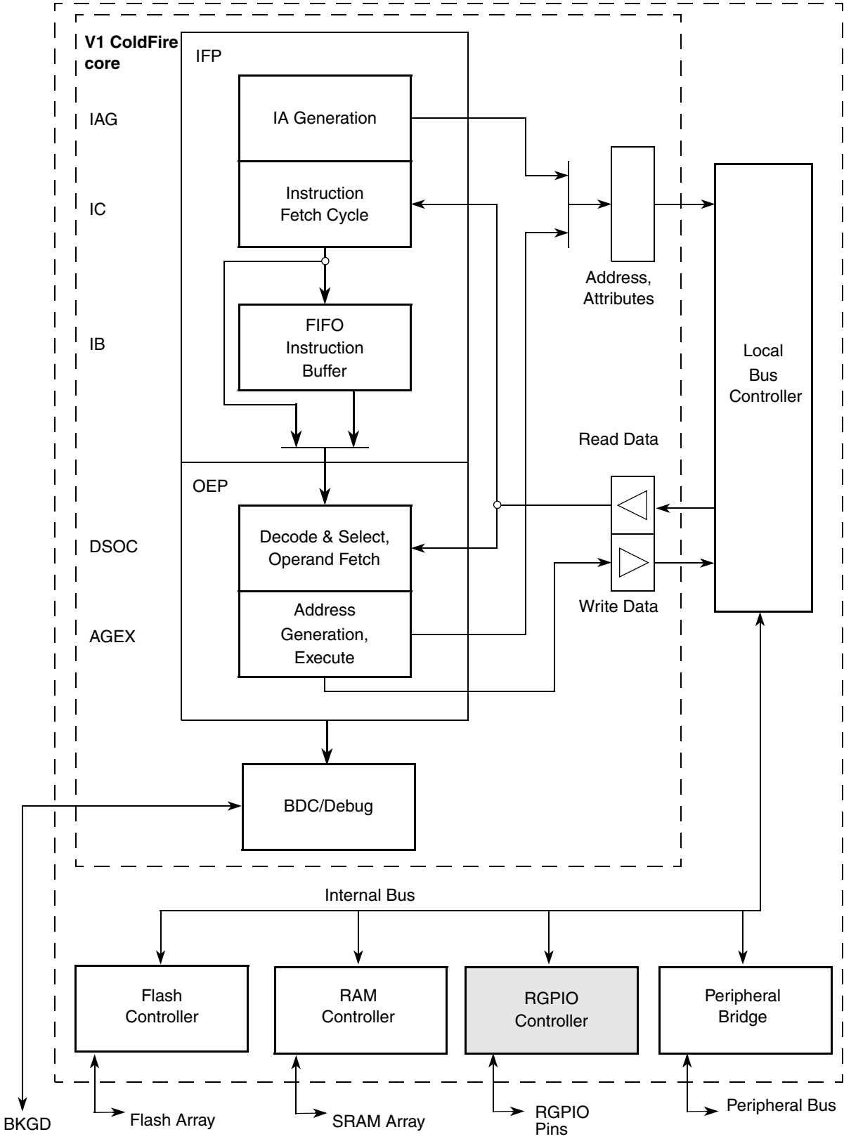
Figure 9-2. V1 ColdFire Block Diagram
