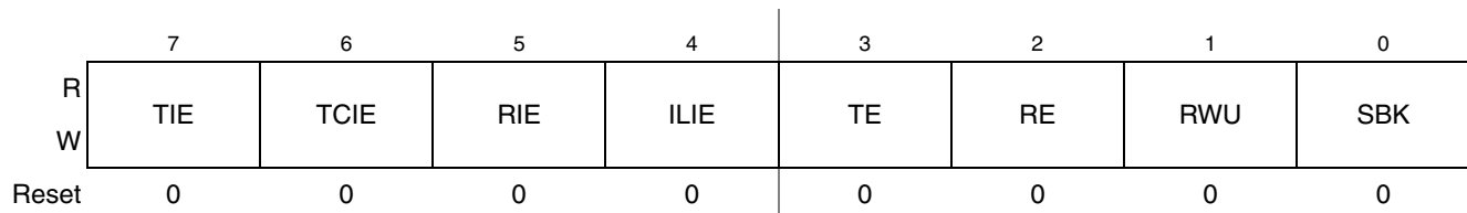
Figure 15-8. SCI Control Register 2 (SC1xC2)
