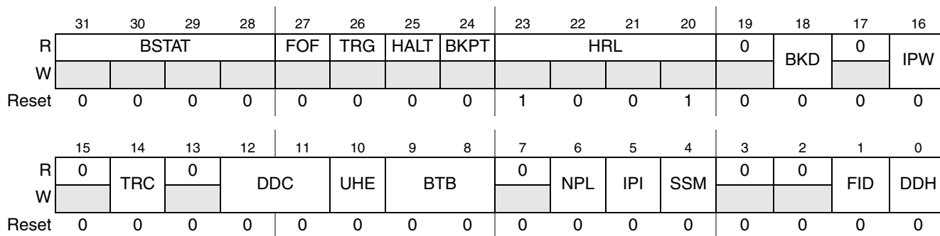
Figure 18-3. Configuration/Status Register (CSR)
