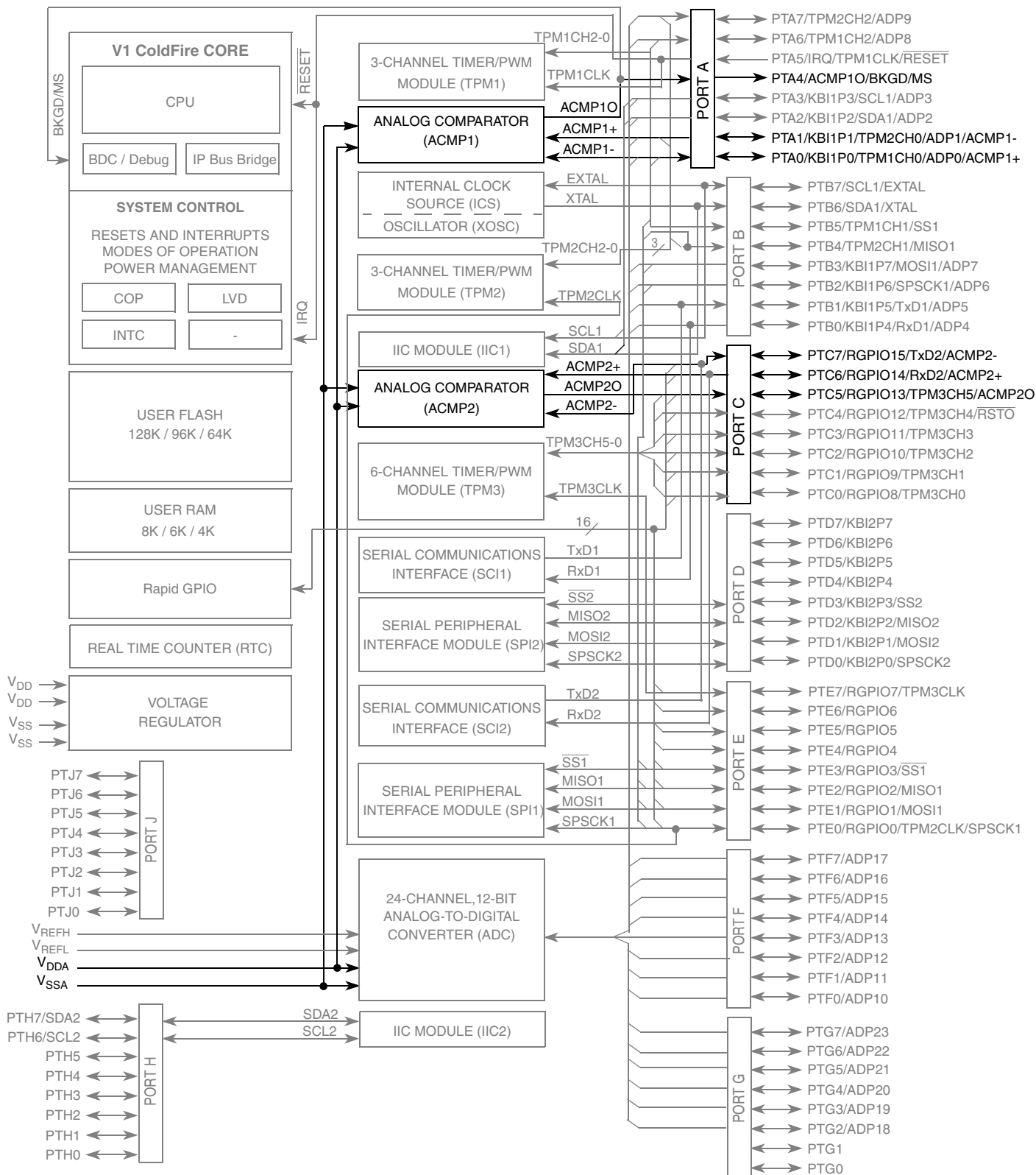
Figure 10-1. MCF51QE128 Series Block Diagram Highlighting ACMP Block and Pins
