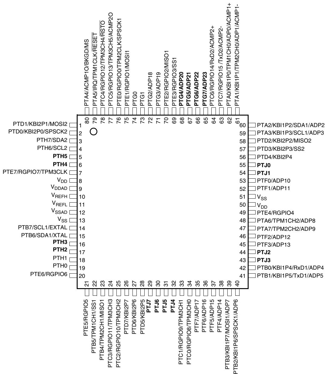
Figure 2-1. 80-Pin LQFP
