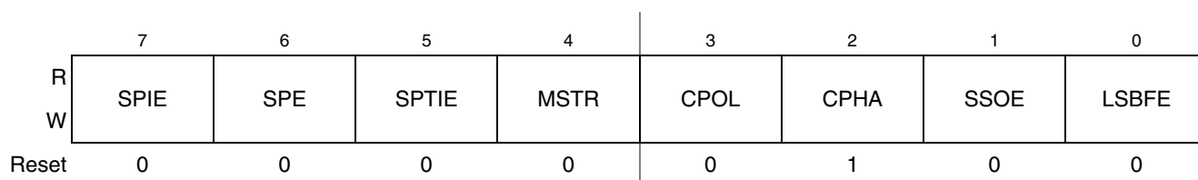
Figure 16-5. SPI Control Register 1 (SPIxC1)
