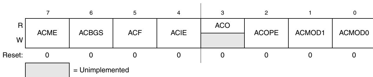
Figure 10-3. ACMP Status and Control Register (ACMPxSC)
