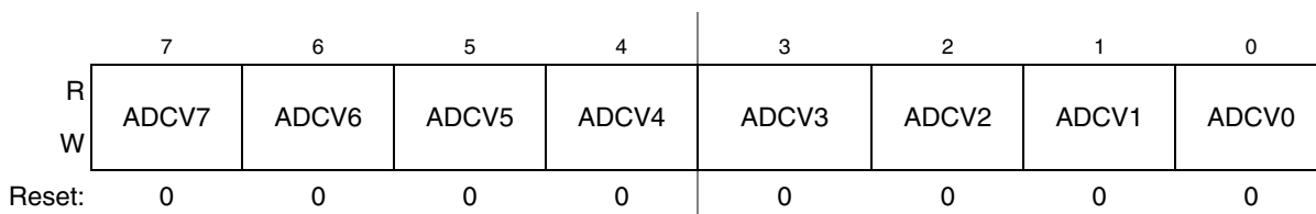
Figure 11-8. Compare Value Low Register(ADCCVL)
