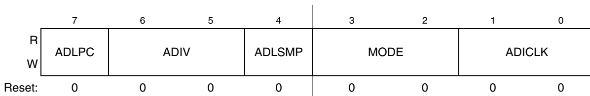
Figure 11-9. Configuration Register (ADCCFG)
