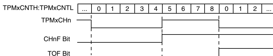
Figure 17-4. Low-True Pulse of an Edge-Aligned PWM
