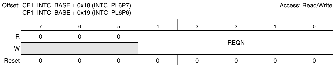
Figure 8-3. INTC_PL6P{7,6} Registers
