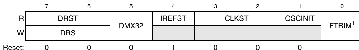
Figure 12-6. ICS Status and Control Register (ICSSC)
