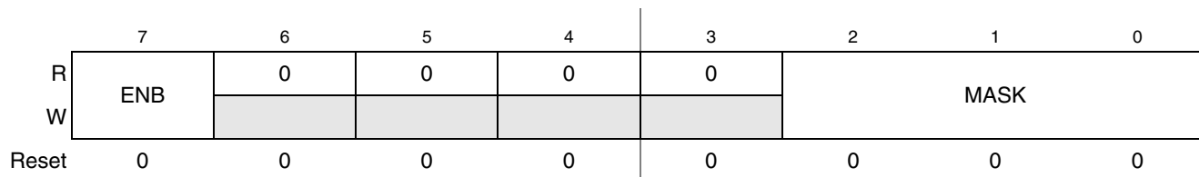
Figure 8-4. INTC_WCR Register
