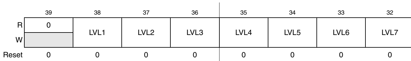
Figure 8-2. INTC_FRC Register
