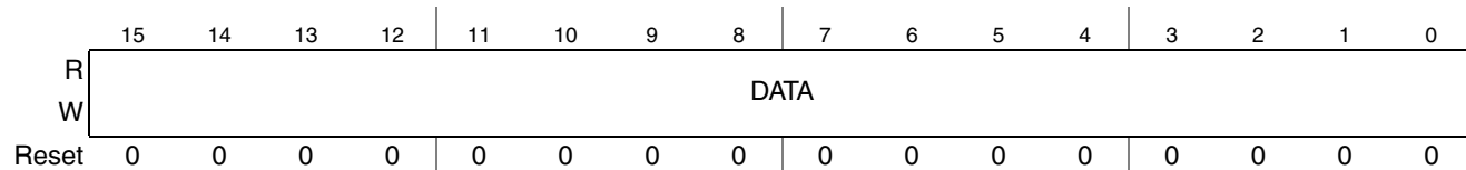
Figure 9-5. RGPIO Data Register (RGPIO_DATA)
