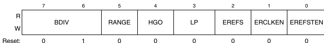
Figure 12-4. ICS Control Register 2 (ICSC2)
