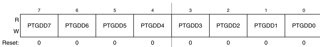
Figure 6-41. Port G Data Direction Register (PTGDD)
