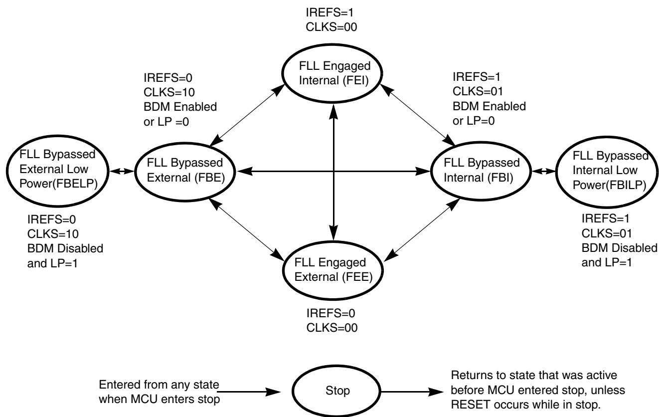
Figure 12-7. Clock Switching Modes
