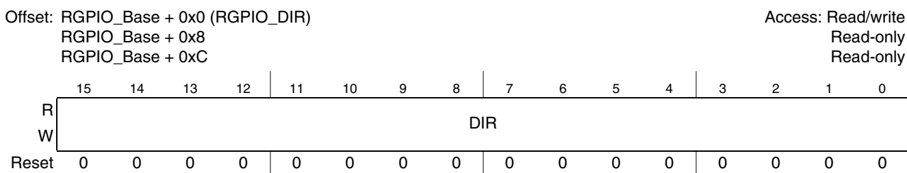
Figure 9-4. RGPIO Data Direction Register (RGPIO_DIR)
