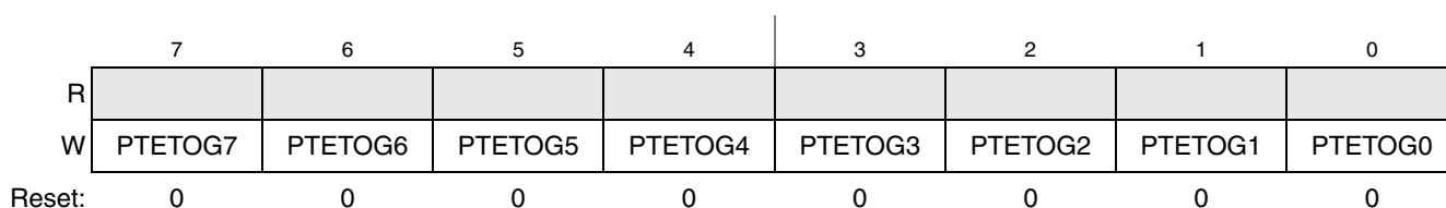
Figure 6-31. Port E Toggle Enable Register (PTETOG)
