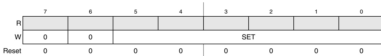
Figure 8-5. INTC_SFRC Register
