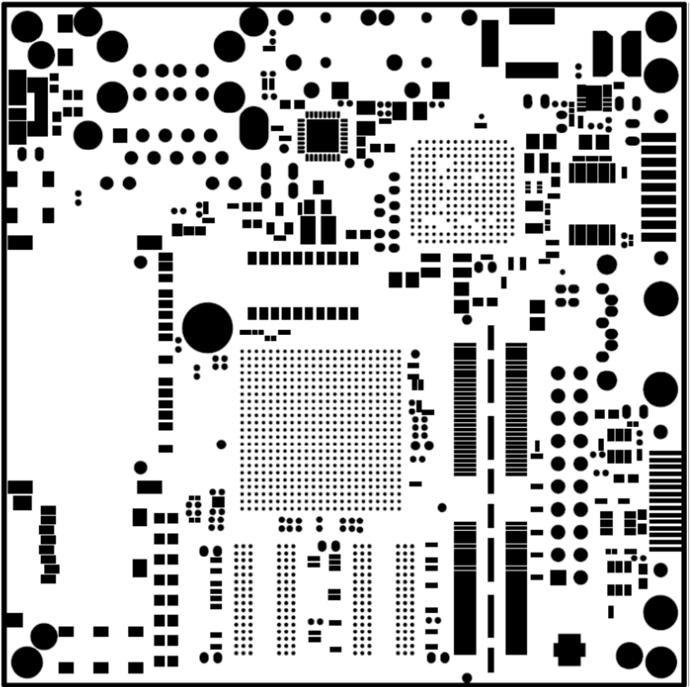
Figure 68. Soldermask Top
