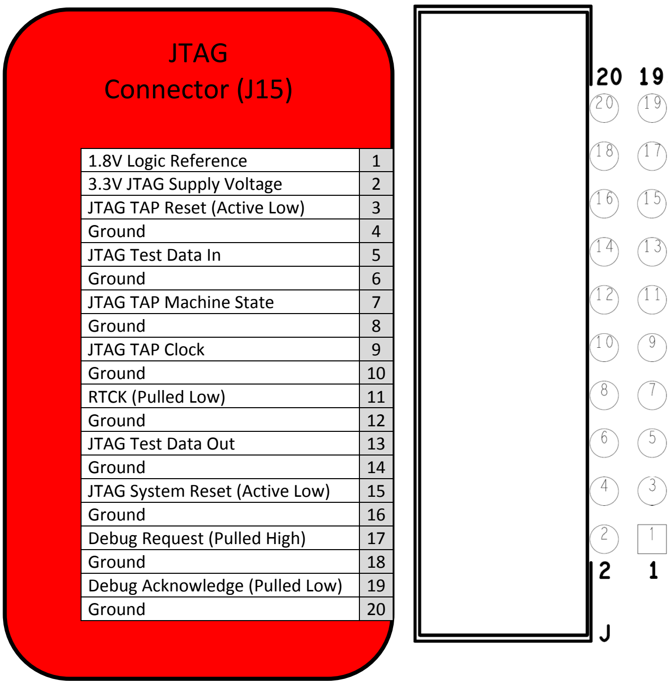
Figure 32. JTAG Connector (J15)
